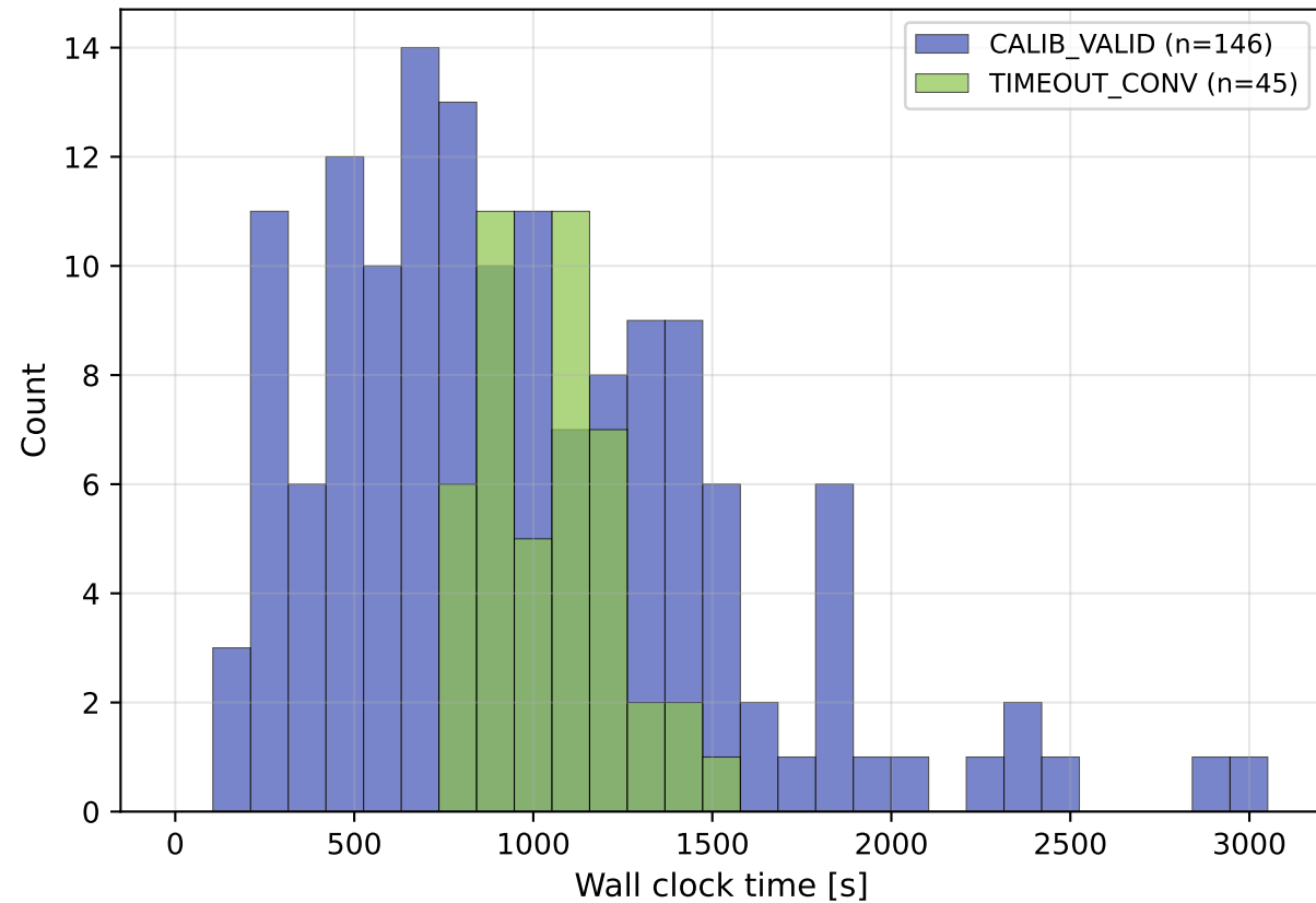
Wall Clock Times TIMEOUT_CONVERGENCE vs CALIB_VALID
