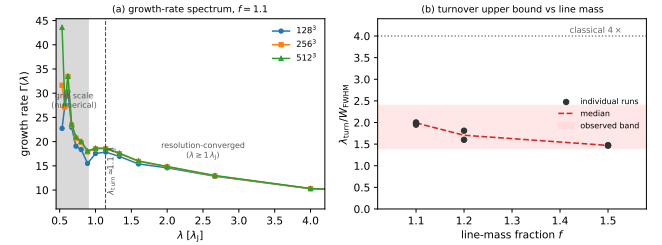
Figure 9. (a) Growth-rate spectrum \Gamma(\lambda) for a near-critical filament ( f = 1.1 ) at three resolutions. For \lambda \gtrsim 1 \lambda_J the curves overlap; at the grid scale (shaded) they separate and rise with resolution. \Gamma plateaus rather than turning over, so \lambda_{\text{turn}} \lesssim 1 \lambda_J is an upper bound . (b) \lambda_{\text{turn}}/W_{\text{FWHM}} against line-mass fraction, in Gaussian FWHM units. The matched, beam-convolved Plummer bound is S_{\text{sim}}^{\text{upper}} \lesssim 1.0\text{--}1.3 (grey band; the \eta_W conversion is uncertain over 0.59\text{--}0.78 , widening it by about a quarter).
