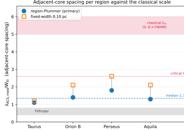
Figure 2. The conditional local descriptor S_{local} = s_{ACS,med}/W_{fil} per primary region. This is not the quantity classical theory predicts (that is S_{global} ; Fig. 4b) and the comparison with the classical band below should be read diagnostically. It is the conditional descriptor measured within core-bearing stretches; the unconditional length per core L/N , whose reciprocal is the line density predicted by fragmentation theory, is shown in Fig. 4, in the two DisPerSE width conventions: directly-measured region-Plummer widths (blue circles, preferred; per-region raw 1.1, 1.4, 1.8, 1.3, dashed line at the median, which we quote as 1.4, the rounded value of the exact median of 1.35) and the fixed 0.10 pc width (orange squares; 1.2, 2.1, 2.6, 2.1), both shown raw (before the injection–recovery correction; Section 2.7). The red band is the classical fastest-growing wavelength \lambda_m \approx 5\text{--}6 \times \text{FWHM} (Fischera & Martin 2012; = 4 \times the flat diameter, Inutsuka & Miyama 1992) and the dotted line the classical critical wavelength \lambda_{cr} \approx 2.6 \times \text{FWHM} ; every region lies well below both. The grey band marks the independent FilFinder skeleton range ( \lambda/W \approx 0.4\text{--}0.8 ). (Uncertainty convention: Section 2.14.)
