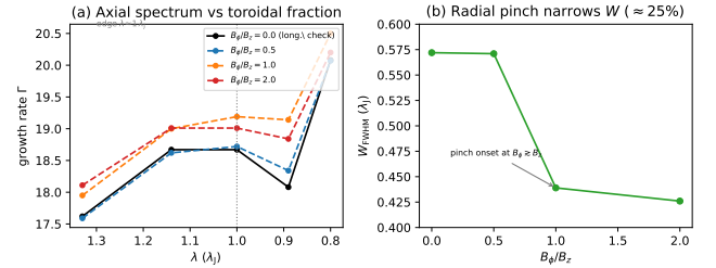
Figure 13. Divergence-free helical-field scan ( B_\phi/B_z = 0 – 2 , 512 \times 128^2 ; Section 4.3). (a) The axial growth-rate spectrum \Gamma(\lambda) in the physical band is invariant to the toroidal fraction ( < 6\% , fit noise), with the converged-band edge fixed at \lambda \approx 1\lambda_J ; B_\phi/B_z = 0 (black) reproduces the pure-longitudinal spectrum, a code check. No excess growth appears at shorter \lambda for any winding. (b) The one systematic effect is a radial pinch : the formation FWHM narrows by \approx 25\% , with onset at B_\phi \gtrsim B_z . The seeded helical field therefore raises \lambda/W by shrinking W , not by shortening \lambda ; the force-balanced Fiege & Pudritz (2000) pinch mode is not tested here.
