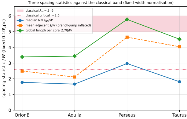
Figure 7. Three spacing statistics per cloud (single reimplementation, all normalised by the fixed 0.10 pc width so they are directly comparable), against the classical band (5–6, red; critical \approx 2.6 , dotted). The median along-skeleton ACS spacing (blue, \approx 1.7 – 3.0 ) is sub-classical everywhere; the global length per core (L/N)/W (green, \approx 3.4 – 5.8 ) is classical in Perseus, near-classical in Taurus, and sub-classical in Orion B and Aquila; the mean adjacent spacing (orange) lies between but is inflated by arclength branch-jumps. The factor- \approx 2 gap between the blue and green points reflects the generic mean/median skew plus dilution by core-poor filament (a coverage effect), not small-scale clustering (Section 2.8): short adjacent spacing within core-bearing stretches, diluted by extensive core-free filament.
