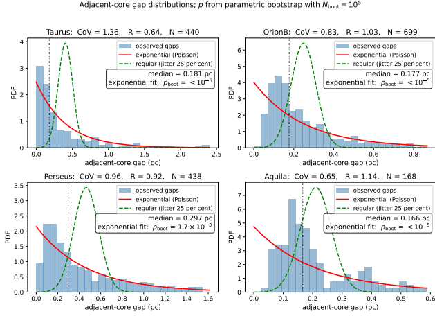
Figure 10. Adjacent-core gap distributions along the skeletons of the four primary regions (histograms), with exponential/Poisson (solid) and regular/periodic (dashed) reference curves; each panel gives the coefficient of variation CoV, the 1-D Clark-Evans ratio R , and the exponential goodness-of-fit p -value calibrated by parametric bootstrap ( p_{\text{boot}} ; the null distribution of the KS statistic is built by resampling from the fitted exponential, removing the estimated-parameter bias of the standard test). The result is two-sided: the regular/periodic model is rejected ( p_{\text{boot}} < 10^{-5} ), the parametric-bootstrap floor, 1/N_{\text{boot}} with N_{\text{boot}} = 10^5 in every region, and the pure-exponential (Poisson) model is also rejected ( p_{\text{boot}} < 10^{-5} (Perseus 1.7 \times 10^{-3} ) in all four), so the cores are neither periodic nor pure-Poisson; consistent with a point process that is locally exclusion-limited but over-dispersed on parsec scales (the deficit of small gaps, R > 1 ; largely instrumental).
