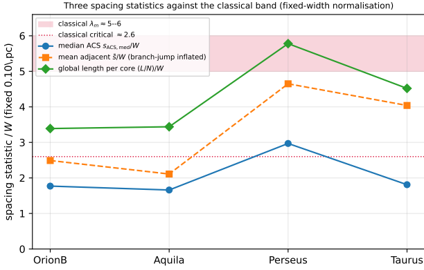
Figure 8. Three spacing statistics per cloud (single re-implementation, all normalised by the fixed 0.10 pc width so they are directly comparable), against the classical band (5–6, red; critical \approx 2.6 , dotted). The median along-skeleton ACS spacing (blue, \approx 1.7 – 3.0 ) is sub-classical everywhere; the global length per core (L/N)/W (green, \approx 3.4 – 5.8 ) is classical in Perseus, near-classical in Taurus, and sub-classical in Orion B and Aquila; the mean adjacent spacing (orange) lies between but is inflated by arclength branch-jumps. The factor- \approx 2 gap between the blue and green points reflects the generic mean/median skew plus dilution by core-poor filament (a coverage effect), not small-scale clustering (Section 2.8): short adjacent spacing within core-bearing stretches, diluted by extensive core-free filament.
