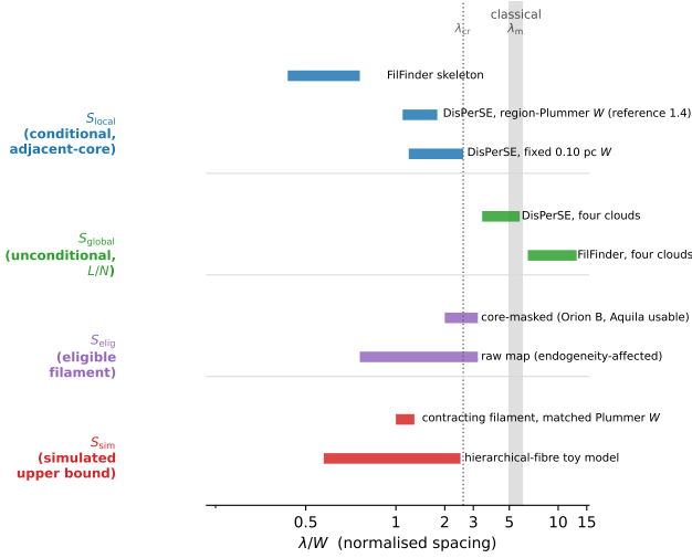
Figure 11. The full methodological envelope of \lambda/W , organised by which quantity is being measured rather than by convention alone. The four groups are the conditional adjacent-core spacing S_{\text{local}} (blue), the unconditional length per core S_{\text{global}} = (L/N)/W (green), the same restricted to fragmentation-eligible filament S_{\text{elig}} (purple; the core-masked row is fiducial, the raw-map row shows the endogeneity-affected comparison), and the simulated upper bound S_{\text{sim}} = \lambda_{\text{turn}}/W together with the hierarchical-fibre toy model (red). Each bar spans the range across clouds and conventions; the grey band is the classical \lambda_m \approx 5-6 (Inutsuka & Miyama 1992; Fischera & Martin 2012) and the dotted line the critical \lambda_{\text{cr}} \approx 2.6 . Grouping this way makes the central point of the paper visible directly: S_{\text{local}} lies well below the classical band under every convention, S_{\text{global}} reaches it, S_{\text{elig}} falls between the two, and S_{\text{sim}} is an upper bound that should not be read as a measured wavelength. Comparisons between groups are comparisons between different quantities and are only meaningful once that is stated (Section 2.16). The horizontal axis is symmetric-log below \lambda/W = 1 .
