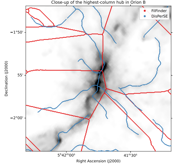
Figure 6. Close-up of the highest-column hub in Orion B, showing FilFinder (red) and DisPerSE (blue) tracks. The two algorithms actually differ. DisPerSE (blue) tracks the visible crests. FilFinder (red) reproduces the main ridge but adds long, nearly straight spokes that radiate from the hub and do not follow the grayscale emission: these are medial-axis artefacts of a large constructed mask rather than resolved sub-filaments. The extra FilFinder length is therefore not obviously tracing real hierarchical structure, which is why we carry the FilFinder branch as the extreme of the convention envelope rather than as an equally-weighted alternative. We stop short of calling FilFinder wrong: a medial axis of a column-density mask is a legitimate and physically motivated definition of a filament network, and deciding which network is real requires velocity information (position–position–velocity data resolving coherent sub-structure), which column density alone cannot supply.
