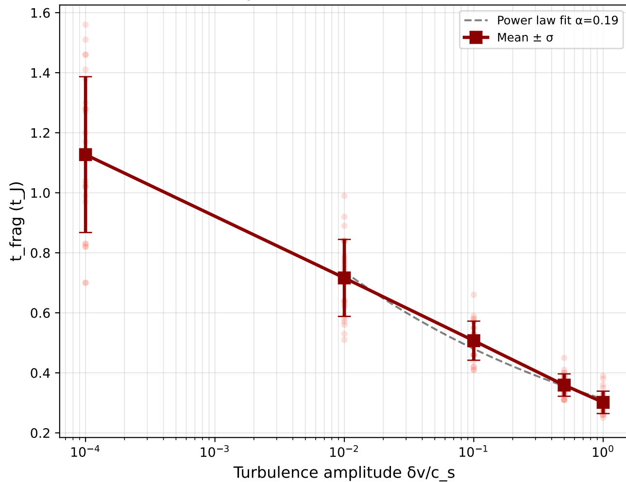
Fragmentation time vs turbulence
