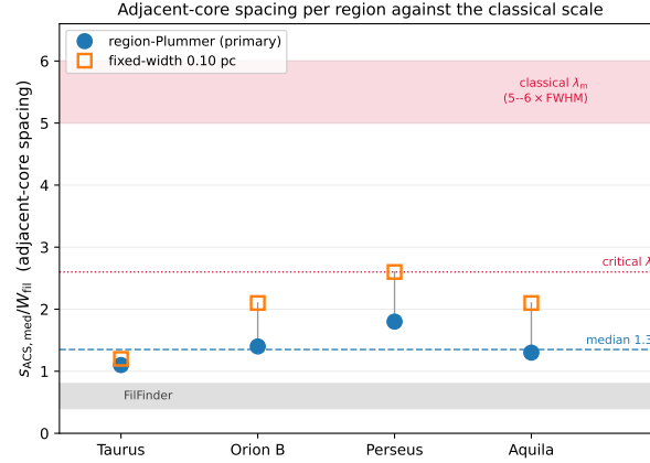
Figure 2. The conditional local descriptor S_{\text{local}} = s_{\text{ACS,med}}/W_{\text{fil}} per primary region. This is not the quantity classical theory predicts (that is S_{\text{global}} ; Fig. 4b) and the comparison with the classical band below should be read diagnostically. It is the conditional descriptor measured within core-bearing stretches; the unconditional length per core L/N , whose reciprocal is the line density predicted by fragmentation theory, is shown in Fig. 4, in the two DisPerSE width conventions: directly-measured region-Plummer widths (blue circles, preferred; per-region raw 1.1, 1.4, 1.8, 1.3, dashed line at the median, which we quote as 1.4, the rounded value of the exact median of 1.35) and the fixed 0.10 pc width (orange squares; 1.2, 2.1, 2.6, 2.1), both shown raw (before the injection–recovery correction; Section 2.7). The red band is the classical fastest-growing wavelength \lambda_m \approx 5\text{--}6 \times \text{FWHM} (Fischera & Martin 2012; = 4 \times the flat diameter, Inutsuka & Miyama 1992) and the dotted line the classical critical wavelength \lambda_{\text{cr}} \approx 2.6 \times \text{FWHM} ; every region lies well below both. The grey band marks the independent FilFinder skeleton range ( \lambda/W \approx 0.4\text{--}0.8 ). (Uncertainty convention: Section 2.14.)
