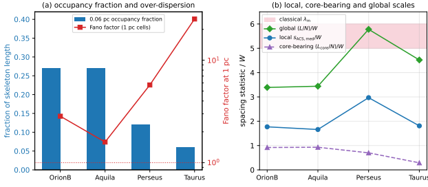
Figure 4. Spatial inhomogeneity of core occurrence along the filaments. (a) The 0.06 pc occupancy fraction (bars, left axis) is 6–27 per cent, while the Fano factor of counts in 1 pc cells (red, right axis, logarithmic) exceeds the Poisson value of unity in every cloud. (b) The three normalised spacing statistics: the local adjacent-core spacing is well below the classical band, the global (L/N)/W approaches it, and the core-bearing (L_{\text{core}}/N)/W lies below both because the occupied stretches are densely populated. The separation between the blue and green curves measures how unevenly the cores occupy the crest.
