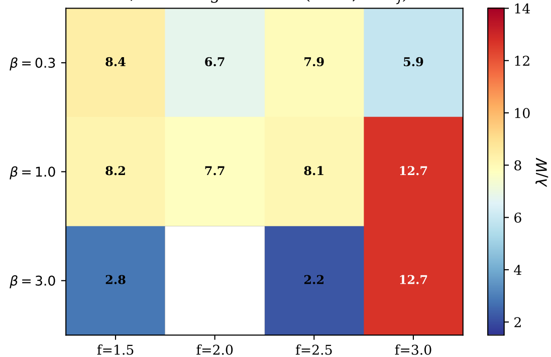
\lambda/W — Longitudinal B ( \theta=0^\circ , 32 \lambda_j )
