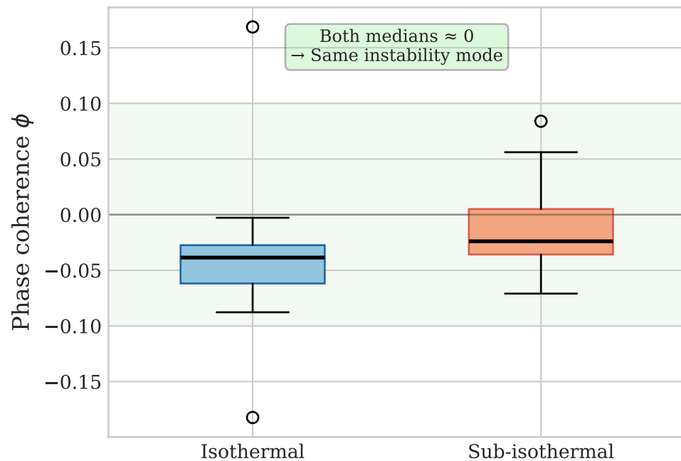
Box Plot
