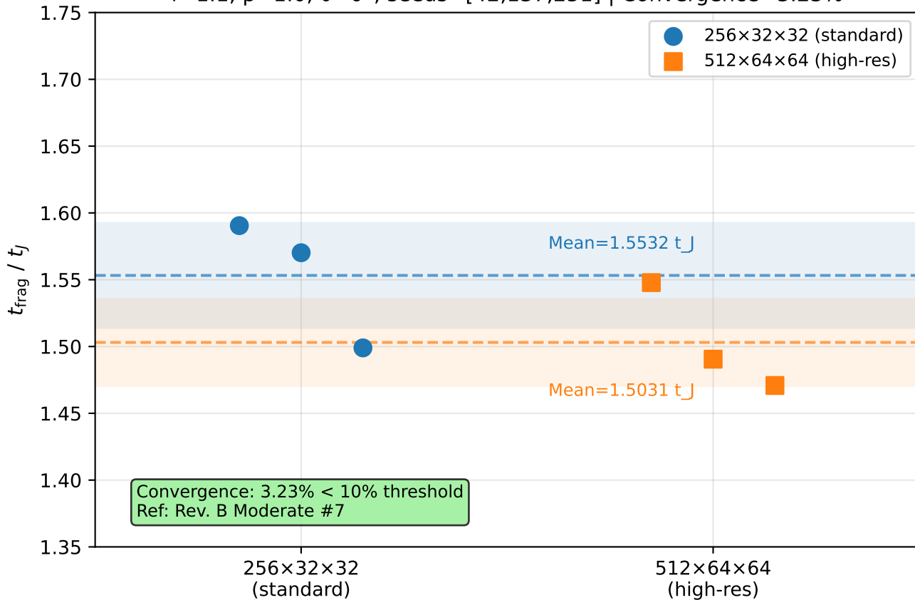
C1: Resolution Convergence Test f=1.1 , \beta=1.0 , \theta=0^\circ , seeds=[42,137,251] | Convergence=3.23%
