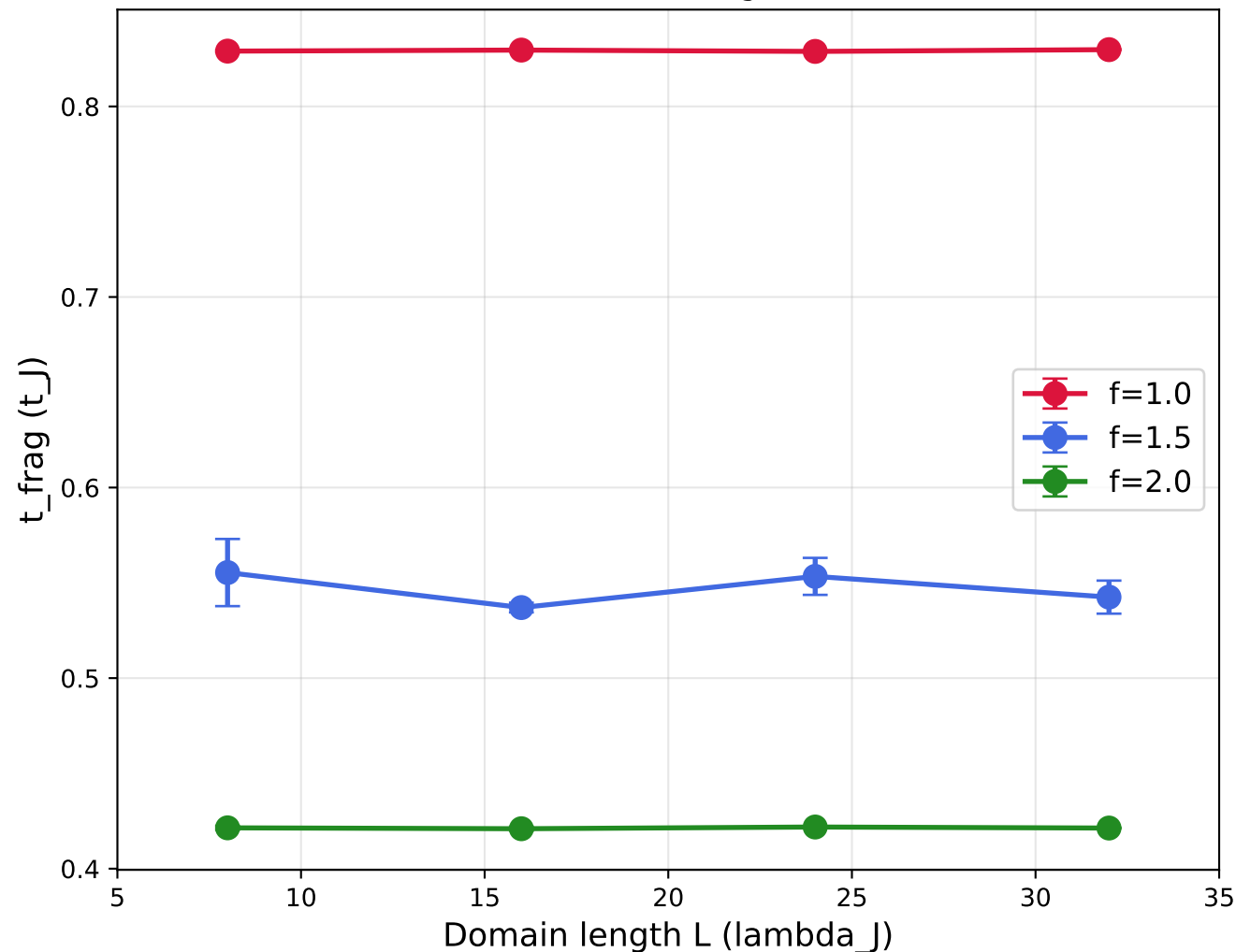
R7: t_{\text{frag}} vs L ( \theta=90 , \beta=1.0 ) Perfect domain convergence at all f
