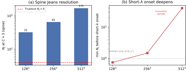
Figure 11. Ideal perpendicular-field refinement ladder ( 128^3 – 512^3 ; Section 4.3). (a) Cells per local Jeans length N_J at the beading-relevant spine contrast C \approx 3 : the collapsing spine is resolved far above the Truelove threshold ( N_J = 4 , dashed) at every resolution. (b) The spurious short- \lambda axial “beading” emerges only once the spine drops below N_J \approx 1 , and refinement pushes that onset to ever-deeper collapse (at 512^3 the filament stays monolithic to N_J \approx 40 at C \approx 30 ); the short- \lambda onset deepening with resolution being the textbook Truelove under-resolution artefact signature, not a physical fragmentation mode.
