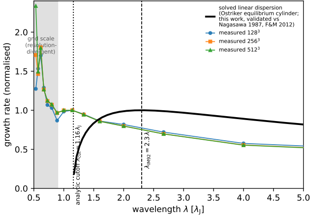
Figure C2. The from-scratch-solved eigenvalue dispersion relation of the isothermal equilibrium cylinder (Nagasawa 1987; Inutsuka & Miyama 1992), validated to < 1% against Nagasawa (1987) and Fischera & Martin (2012) (not a fit): it peaks at \lambda_{\text{IM92}} \approx 2.3 \lambda_J and vanishes at the cutoff \lambda_{\text{cr}} \approx 1.2 \lambda_J , overplotted on the measured growth-rate spectrum ( f = 1.1 , three resolutions, normalised at \lambda = 1.14 \lambda_J ). The measured spectrum instead rises monotonically into the grid-scale region (shaded), confirming the small-scale rise is numerical, so the measured \approx 1.1 \lambda_J wavelength is an order- \lambda_J , sub-classical value, not a precisely-located maximum.
