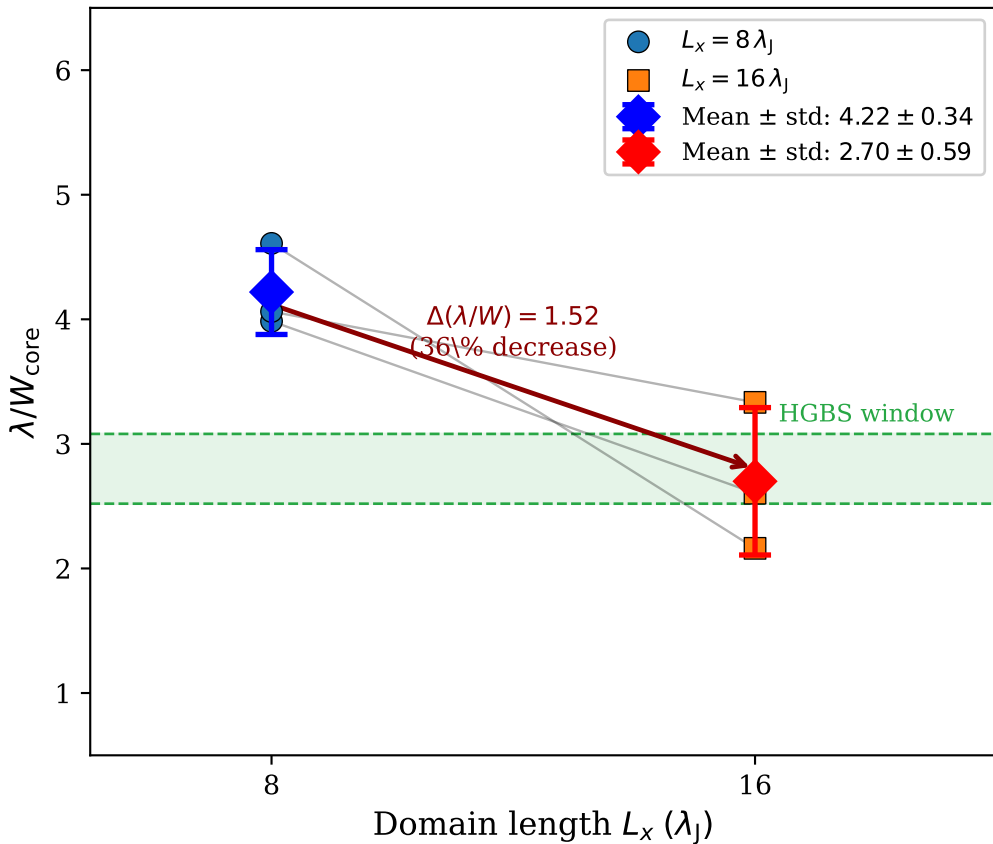
Box-size convergence ( f = 2.6 , \beta = 1.0 )
