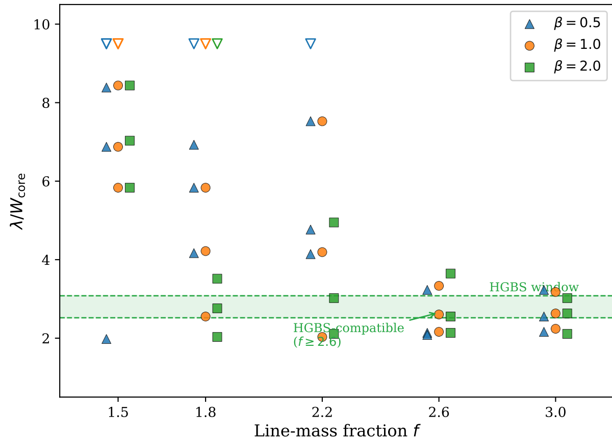
Rigid Cylinder Campaign: fragmentation spacing vs f
