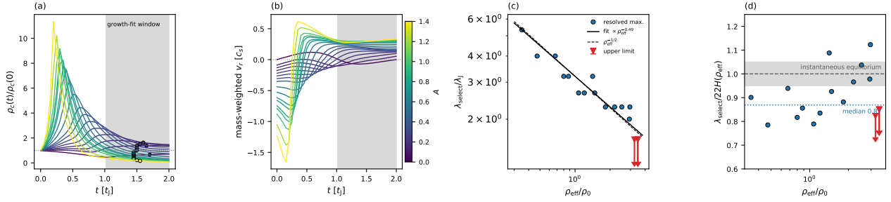
Figure 4. The impulsive-contraction ladder: seventeen runs, coloured by the imposed inward-velocity amplitude A . (a) Central density against time, normalised to its initial value; the shaded band is the window over which the growth rates are fitted, and the circles mark the epoch at which \rho_{\text{eff}} is evaluated. The overshoot and rebound are visible directly: a strong kick raises the density transiently and leaves the filament less dense than it started while its modes are growing. (b) Mass-weighted radial velocity within 0.6\lambda_J of the axis, showing the same behaviour. (c) Selected scale against \rho_{\text{eff}} . Circles are runs with a resolved maximum of \Gamma ; triangles are upper limits, where \Gamma is still rising at the shortest well-resolved seeded mode. The solid line is the censored maximum-likelihood fit (Eq. 10) and the dashed line the \rho_{\text{eff}}^{-1/2} expectation. (d) The same selected scale normalised by the equilibrium result evaluated at each run’s own \rho_{\text{eff}} rather than at the initial density. Once the changing background is removed the residual shift is small: the static run sits at 1.09 and the dynamical runs have a median of 0.87, so the deficit relative to the instantaneous equilibrium expectation is of order 13 per cent, an order of magnitude smaller than the factor of three to five obtained by comparing with the initial equilibrium wavelength.
