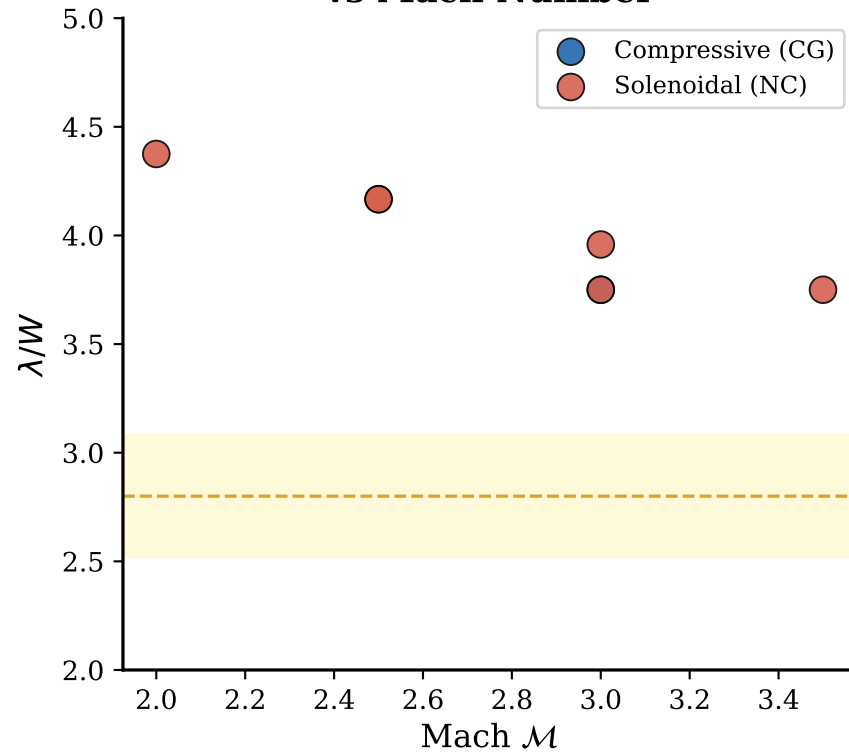
HGBS-Proximate Events vs Mach Number
