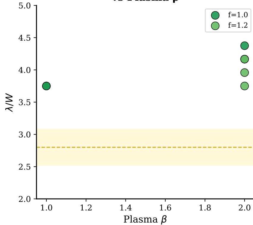
HGBS-Proximate Events vs Plasma \beta
