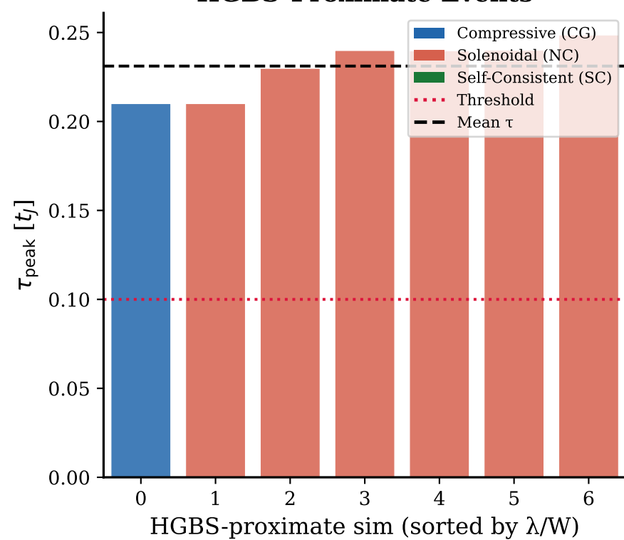
Peak Survival for HGBS-Proximate Events
