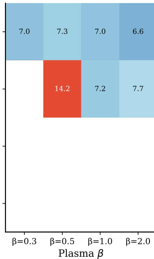
Self-Consistent (SC)
