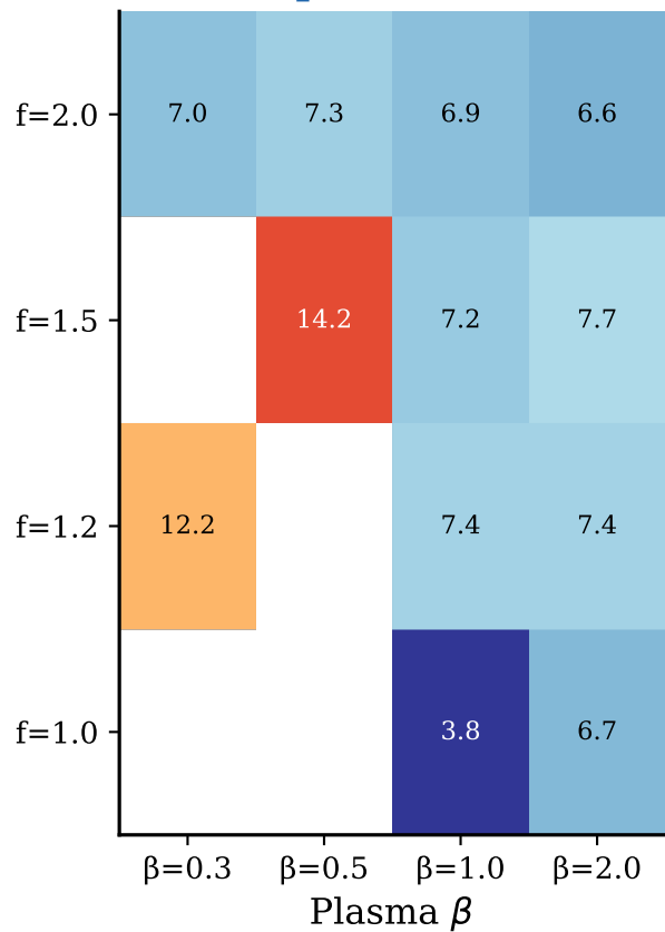
Compressive (CG)
