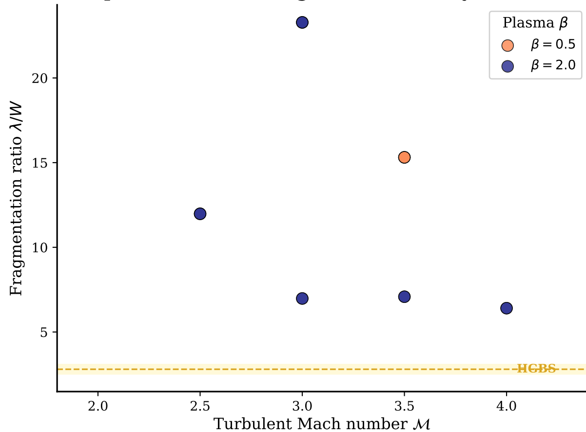
Perpendicular Field Fragmentation at Physical Mach
