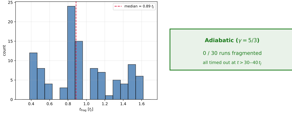
Figure 8. Equation-of-state dependence. Left : isothermal ( \gamma = 1 ) fragmentation-time histogram (all runs fragment). Right : adiabatic ( \gamma = 5/3 ) all-null annotation, 0/30 runs fragmented, all timed out at t > 30 – 40 t_J (no distribution is meaningful for a 0/30 outcome, so the panel states the result textually).
