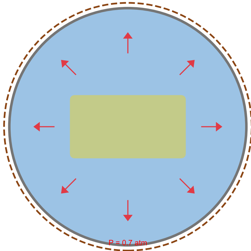
Turgor Pressure Mechanism for Bacterial Cell Division
