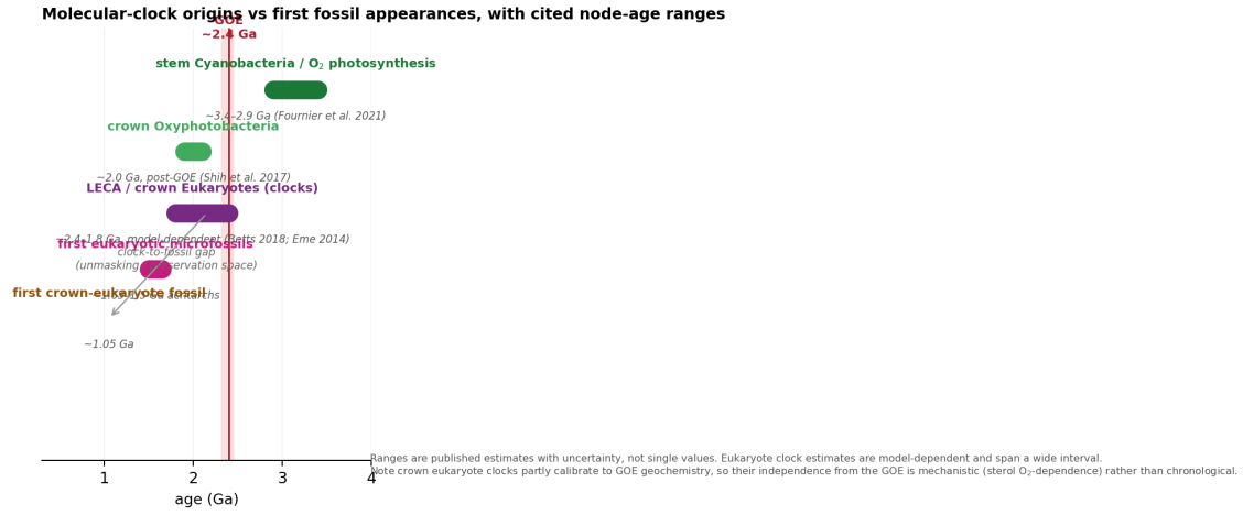
Figure 4: Molecular clock estimates of lineage origin against first fossil appearances, with published node-age ranges. The stem origin of cyanobacteria lies in the Archaean (Fournier et al., 2021); crown Oxyphotobacteria diversify around or after the GOE (Shih et al., 2017); eukaryote estimates are model-dependent (Betts et al., 2018; Eme et al., 2014) and partly calibrated to GOE geochemistry.
