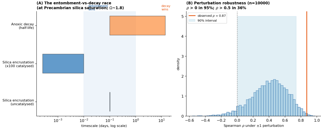
Figure 2: (A) The entombment–decay race at Precambrian silica saturation ( \Omega \approx 1.8 ). Abiotic silica encrustation (Rimstidt & Barnes, 1980) rate law deposits a 100 nm layer in \approx 1 hour, one to two orders of magnitude faster than anoxic decay (3–14 days). Surface catalysis or inhibition introduces large uncertainty. (B) Perturbation robustness: with \pm 1 random noise on all scores, the silicification–fidelity Spearman \rho remains positive in 95% of 10,000 perturbations, confirming the direction of the association is robust to coding subjectivity.
