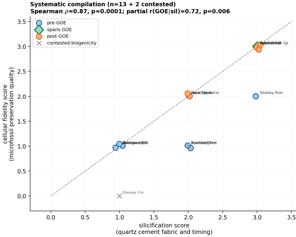
Figure 1: Systematic compilation of 15 Precambrian chert-hosted microfossil biotas. Silicification score (from quartz cement fabric and timing, coded independently of fidelity) against cellular fidelity score. Spearman \rho = 0.87 , p < 0.001 ( n = 13 accepted biogenicity; n = 15 including contested). GOE position retains significant explanatory power after controlling for silicification (partial r = 0.72 , p = 0.006 ), indicating a residual GOE-associated signal in fidelity whose origin cannot be resolved from this compilation. Crosses = contested biogenicity (Apex, Dresser), included for sensitivity but excluded from the primary analysis.
