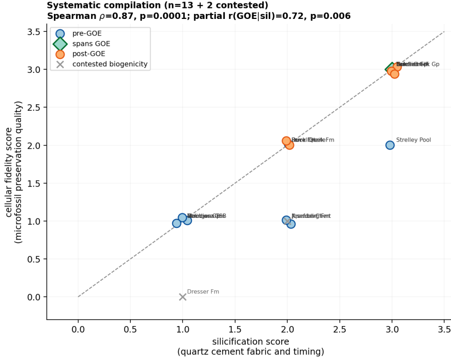
Figure 2: Systematic compilation of 15 Precambrian chert-hosted microfossil biotas. Silicification score (from quartz cement fabric and timing, coded independently of fidelity) against cellular fidelity score. Spearman \rho = 0.87 , p < 0.001 ( n = 13 accepted biogenicity; n = 15 including contested). GOE position retains a residual association with fidelity after controlling for silicification (partial r = 0.72 ; bootstrap 95% CI: 0.13–0.94). Note: some formation labels overlap in this figure; refer to Table 1 for exact scores and sources. Crosses = contested biogenicity (Apex, Dresser), included for sensitivity but excluded from the primary analysis.
