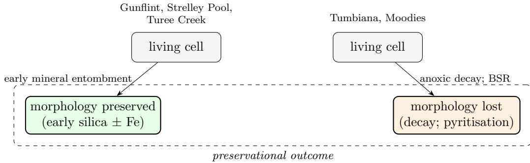
Figure 4: Preservational pathways. Where early mineral entombment outpaces decay, morphology is retained; where decay precedes mineralisation, morphology is lost and kerogen survives.
