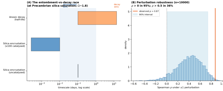
Figure 1: The entombment–decay race at Precambrian silica saturation ( \Omega \approx 1.8 ). Abiotic silica encrustation (Rimstidt & Barnes, 1980) rate law deposits a 100 nm layer in \approx 1 hour, one to two orders of magnitude faster than anoxic decay over days to weeks (Corth  sy et al., 2025). Surface catalysis or inhibition introduces large uncertainty in the effective rate constant. The inset perturbation histogram addresses coding noise but not the shared-provenance circularity discussed in the text.
