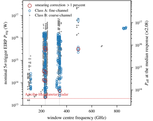
FIG. 9.— Two-dimensional sensitivity against window centre frequency for all 1655 searched windows, symbol by channelisation class, the axis along which completeness differs (Table 12). Left axis : the nominal trigger threshold P_{\text{trig}} , an internal detection statistic. Right axis : the effective threshold at the median response, P_{\text{eff}} = 2.08 P_{\text{trig}} , which is the power to compare with a transmitter (§4); the per-window ratio P_{\text{eff},\text{total}}/P_{\text{trig}} runs 1.33–3.63, so a single window’s threshold should be read from the catalogue, not from this axis. Red rings mark the 9 windows whose smearing correction exceeds 1 per cent; dotted, the Arecibo 2.38-GHz benchmark. Note the two decades of scatter at fixed frequency: there is no single survey sensitivity.
