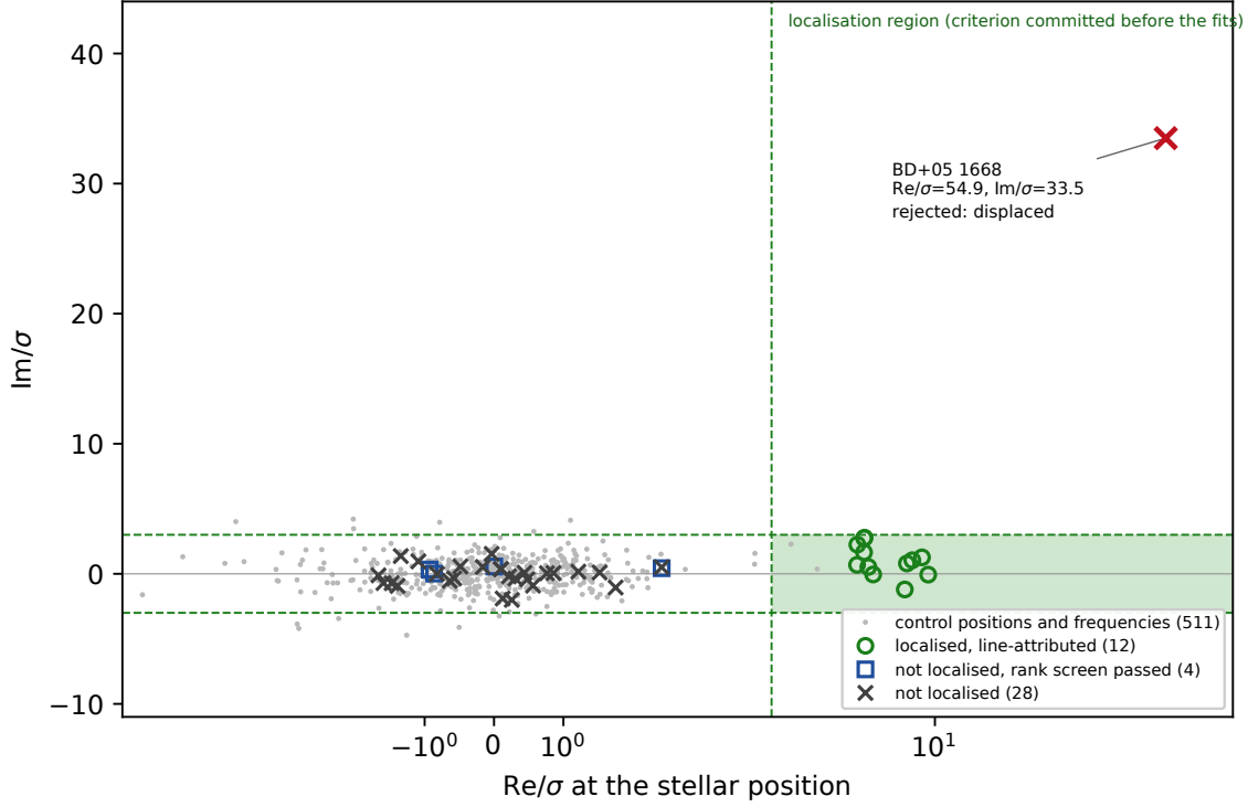
FIG. 5.— The visibility-domain localisation of every threshold crossing that could be fitted, in units of the measurement uncertainty: the real part of the visibility phase-rotated to the stellar position against its imaginary part. Emission centred on the star makes the real part positive and significant and leaves the imaginary part at zero; emission displaced from the phase centre does not. Grey points are the control positions and control frequencies of the same fits, which carry no event by construction and show the null. The shaded region is the localisation criterion, fixed and committed at edfcc0d3d7db before any of these fits was run. 12 crossings fall inside it and the frozen line mask attributes every one of them to carbon monoxide; 0 are unattributed. The crossings the rank screen passed are marked separately: 4 crossings it rejected are localised here, and 4 it passed are not.
