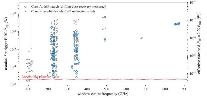
FIG. 6.— Two-dimensional sensitivity against window centre frequency for all 443 searched windows, symbol by channelisation class, the axis along which completeness differs (Table 3). Left axis : the nominal trigger threshold P_{\text{trig}} , an internal detection statistic. Right axis : the effective threshold P_{\text{eff}} = 2.29 P_{\text{trig}} , which is the power to compare with a transmitter (§4). Ringed symbols are the 9 windows whose intra-integration smearing correction exceeds 1 per cent. Grey lines mark the Bands 3, 6 and 7 concentrations; dotted, the Arecibo 2.38-GHz EIRP benchmark, a power scale only. Note the two decades of scatter at fixed frequency: there is no single survey sensitivity.
