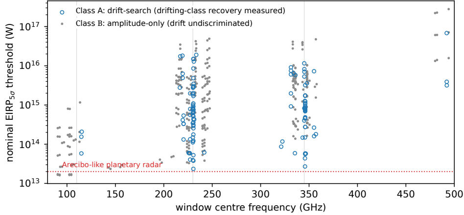
FIG. 9.— Two-dimensional sensitivity of this release: nominal EIRP trigger threshold (boxed rule, §4) against window centre frequency for all 431 searched windows, symbol by channelisation class, the axis along which completeness differs (Table 18). Grey lines mark the Bands 3, 6 and 7 concentrations; dotted, Arecibo-class power.
