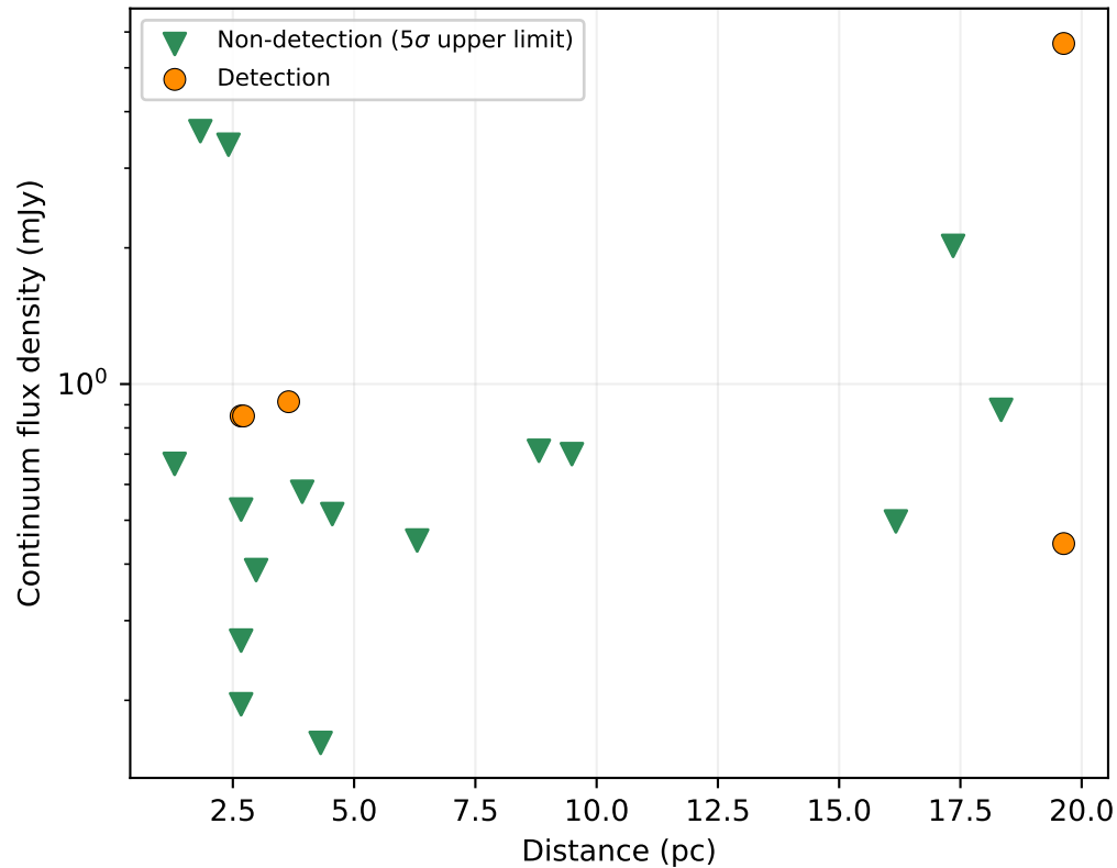
Continuum sensitivity
