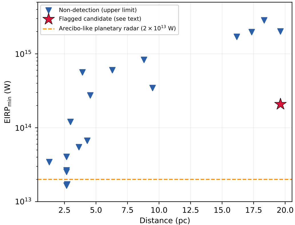
Technosignature sensitivity
