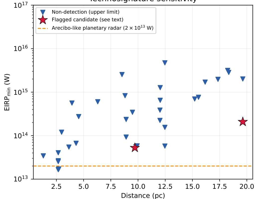
Technosignature sensitivity
