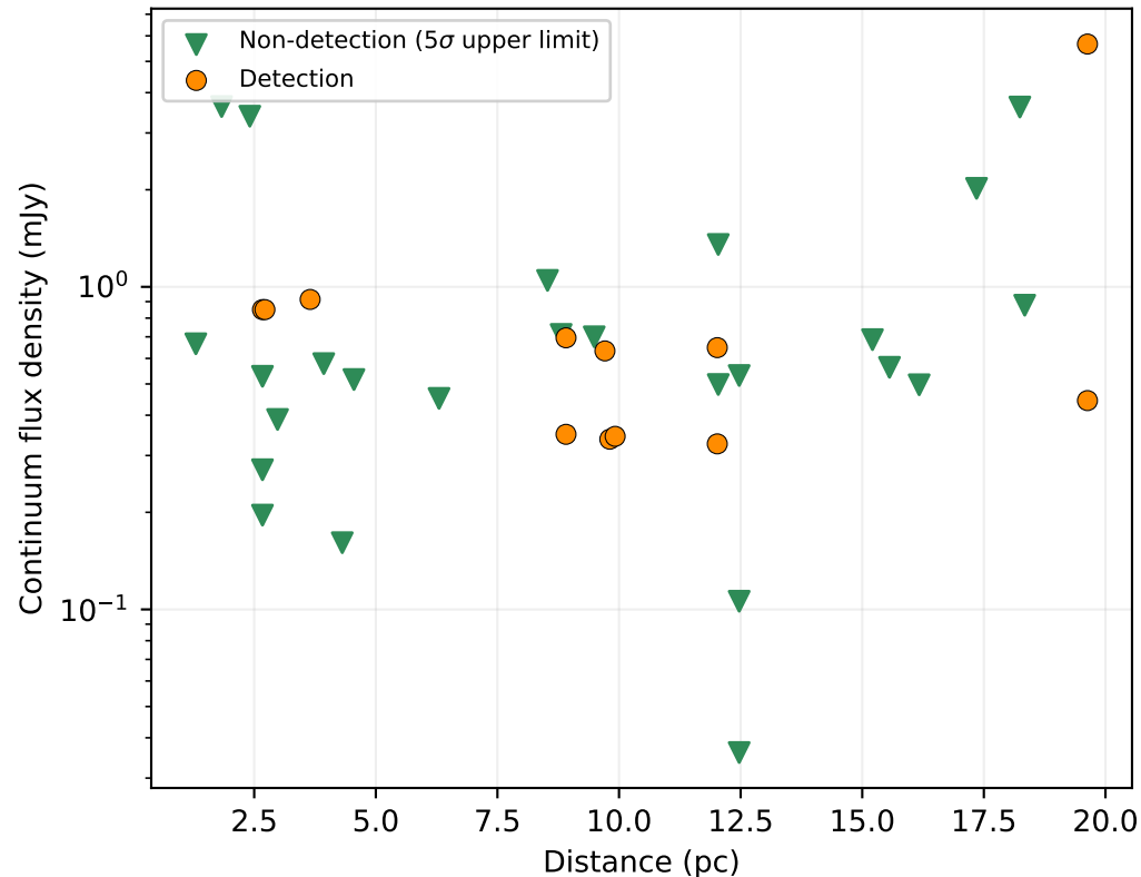
Continuum sensitivity
