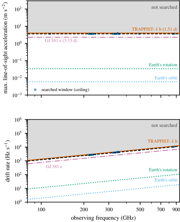
FIG. 6.— What the drift search reaches, as a physical selection function. Upper : the drift ceiling of each of the 403 Class A windows (points), converted to line-of-sight acceleration, |a| = c\dot{\nu}/\nu , against observing frequency; shaded above is unsearched. The boundary is flat because the grid was built at constant acceleration, 3.60 \text{ m s}^{-2} . Lower : the same boundary in the units the search works in, where it is not flat, running 1.4 \text{ kHz s}^{-1} at 115 GHz to 10.5 \text{ kHz s}^{-1} at 872 GHz. Horizontal lines are reference accelerations: Earth’s rotation ( 0.034 \text{ m s}^{-2} at the equator) and orbit ( 0.0059 \text{ m s}^{-2} ), and the two most demanding known planets of any target, TRAPPIST-1 b ( 4.00 \text{ m s}^{-2} ) and GJ 581 e ( 2.27 \text{ m s}^{-2} ). TRAPPIST-1 b is the one case the grid does not contain, missing by 0.01 per cent.
