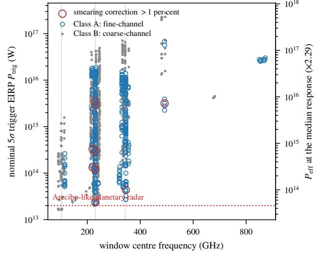
FIG. 10.— Two-dimensional sensitivity against window centre frequency for all 1655 searched windows, symbol by channelisation class, the axis along which completeness differs (Table 12). Left axis : the nominal trigger threshold P_{\text{trig}} , an internal detection statistic. Right axis : the effective threshold at the median response, P_{\text{eff}} = 2.29 P_{\text{trig}} , which is the power to compare with a transmitter (§4); the per-window ratio P_{\text{eff, total}}/P_{\text{trig}} runs 1.33–3.98, so a single window’s threshold should be read from the catalogue, not from this axis. Red rings mark the 9 windows whose smearing correction exceeds 1 per cent; dotted, the Arecibo 2.38-GHz benchmark. Note the two decades of scatter at fixed frequency: there is no single survey sensitivity.
