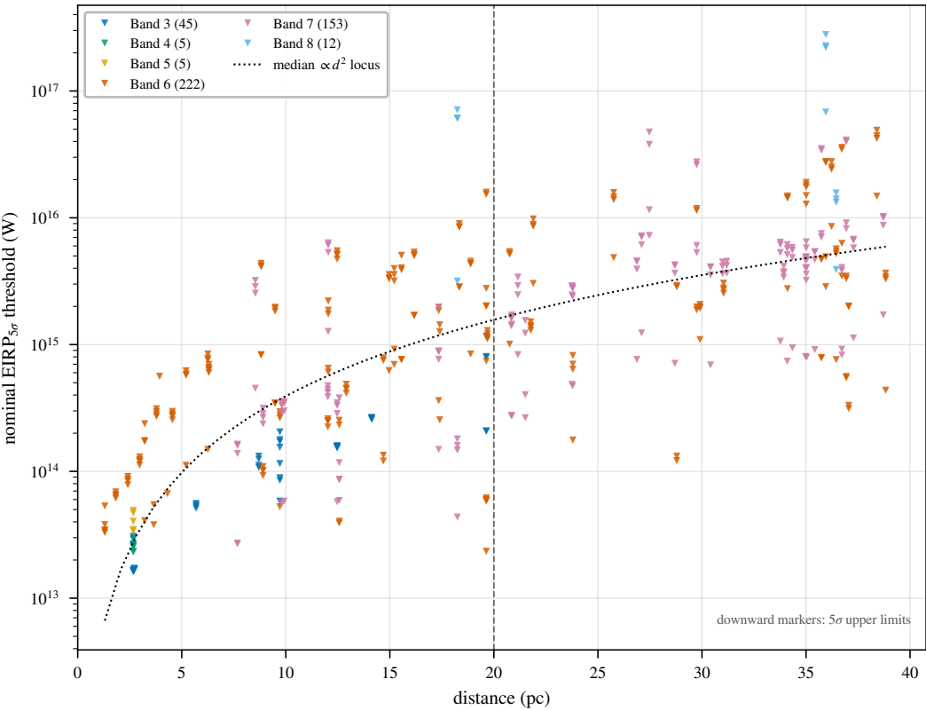
(a) narrowband transmitter limit (upper limits)
