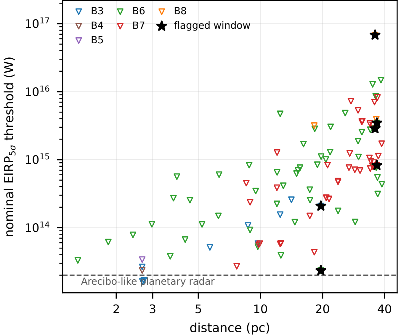
FIG. 8.— Nominal \text{EIRP}_{5\sigma} thresholds (boxed rule, §4) against distance, one deepest window per star and band (104 datasets, 85 stars); every point is an upper limit. Stars mark the four windows with a spatially significant hit (Table 5). The dashed line is an Arecibo-like planetary radar, 2 \times 10^{13} W, a scale for human transmitter power and not a claim that the survey reaches Earth-technology detectability (§4.3).
