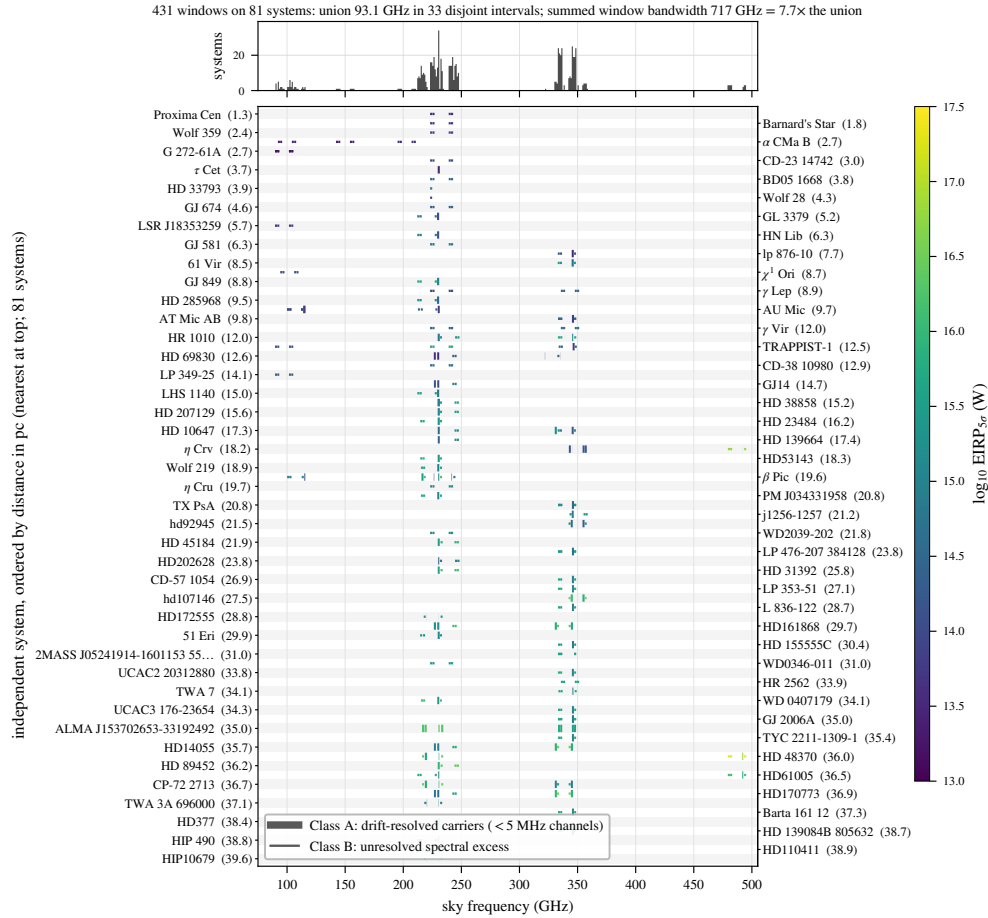
FIG. 3.— What this survey sampled in frequency. Each searched window is a horizontal segment on its host system’s row, rows ordered by distance, coloured by nominal EIRP 5 \sigma , with line weight distinguishing the drift-resolved (Class A) from the unresolved-spectral-excess (Class B) channelisation; the upper panel counts systems per gigahertz of sky frequency. The coverage is narrow, clustered and repeatedly revisited: 33 islands concentrated near 230 and 345 GHz, with summed window bandwidth 7.7 \times the union, which is what the in-band transmitter fractions of Appendix I condition on (Scope of the constraints, §4).
