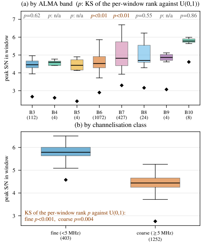
FIG. 10.— Exchangeability of the 512-position control ensemble by stratum, over 1655 windows. Boxes give the per-window control maximum, black diamonds the median on-star peak, and p the Kolmogorov–Smirnov test of the per-window rank against U(0, 1) . (a) by ALMA band, with the window count under each label; (b) by channelisation class, fine ( < 5 MHz) against coarse. The ensemble tracks the on-star statistic in every band and both channelisation classes. The one departure is the drift-search class ( p = 0.015 ), driven by the 13 flagged windows of Table 7.
