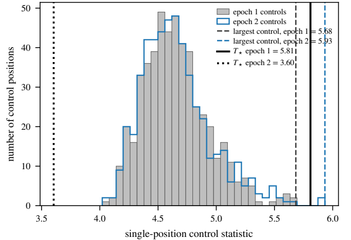
FIG. 14.— The CP–72 2713 Band 7 crossing inside its own control ensemble, in both executions. Histograms give the 512 single-position control statistics of that window in execution 1 (filled) and in the second block 2.05 h later (outline); the two agree, which is the evidence that the datasets are comparable. Vertical lines mark T_\star and the largest control in each. In execution 2 the control annulus alone reaches 5.93, beyond the 5.81 that raised the flag, while the star falls to 3.60.
