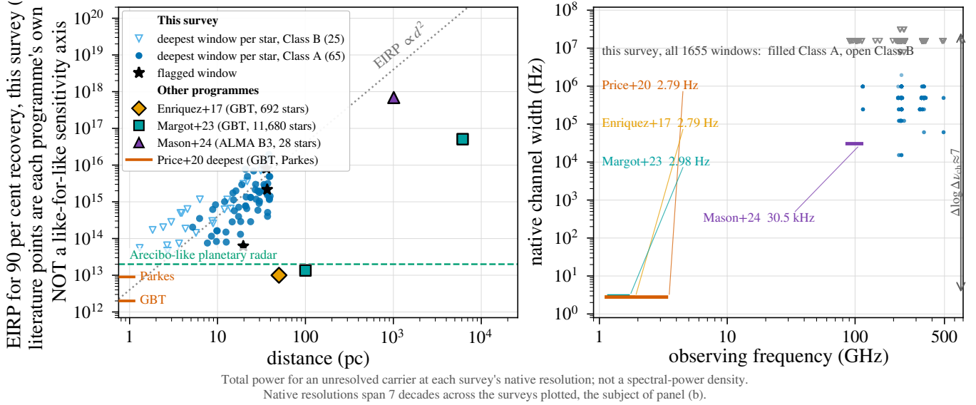
FIG. 1.— Literature context of the 5σ trigger thresholds, in total power (§2). (a) EIRP against distance. Blue: this survey, plotted as P_{90} , the power recovered in 90 per cent of injection trials, for the deepest window per star (90 stars, 1.30–39.63 pc; filled: Class A, fine-channel; open: Class B, coarse-channel); orange: Enriquez et al. (2017); aqua: Margot et al. (2023); violet: Mason et al. (2024); left-edge ticks: deepest per-target limits of Price et al. (2020). Grey dotted: \text{EIRP} \propto d^2 at constant received flux. Green dashed: the Arecibo 2.38-GHz EIRP benchmark, a power scale only (§4.3). (b) Native channel width against observing frequency for the same windows and programmes: resolutions differ by \sim 10^7 , so the panels must be read together and a lower EIRP here does not imply greater sensitivity to a hertz-wide carrier. This is not a like-for-like sensitivity comparison , and the ordinate says so. This survey is plotted at 90 per cent measured recovery; the literature points are each programme’s own 5σ threshold statistic, and those differ in definition, in the channel width they are evaluated over, and in the completeness they correspond to. We know of no way to convert the published values to a common completeness, so the comparison should be read as approximate. A further \times 1.41 is available to this survey from the individual parallel hands and is not taken here.
