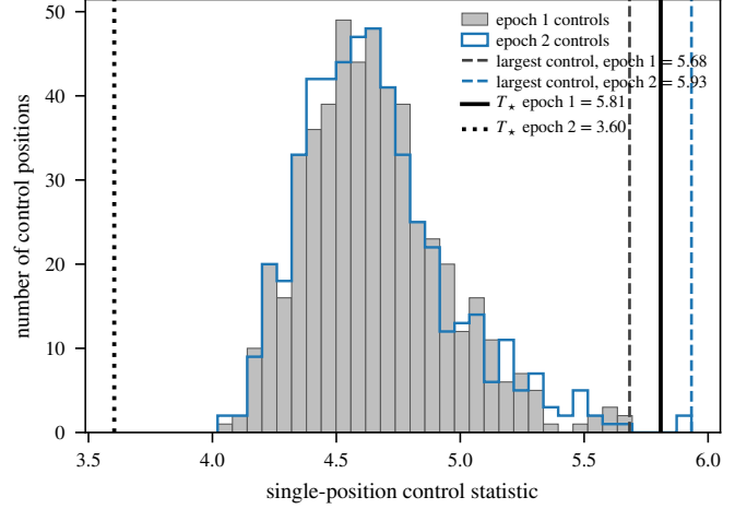
FIG. 8.— The CP-72 2713 Band 7 crossing inside its own control ensemble, in both executions. Histograms give the 512 single-position control statistics of that window in execution 1 (filled) and in the second block 2.05 h later (outline); the two agree, which is the evidence that the datasets are comparable. Vertical lines mark T_\star and the largest control in each. In execution 2 the control annulus alone reaches 5.93, beyond the 5.81 that raised the flag, while the star falls to 3.60.
