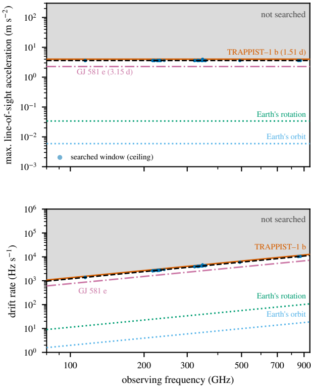
FIG. 12.— What the drift search does and does not reach, as a physical selection function. Upper : the drift ceiling of each of the 403 Class A windows (points), converted to the line-of-sight acceleration it corresponds to, |a| = c\dot{\nu}/\nu , against observing frequency; shaded above is unsearched. The boundary is flat because the grid was built at constant acceleration, 3.60 \text{ m s}^{-2} , and not at constant drift rate. Lower : the same boundary in the units the search works in, where it is not flat: the same 3.60 \text{ m s}^{-2} is 1.4 \text{ kHz s}^{-1} at 115 GHz and 10.5 \text{ kHz s}^{-1} at 872 GHz. Reference accelerations, all frequency-independent and so horizontal in the upper panel: Earth's rotation ( 0.034 \text{ m s}^{-2} at the equator) and orbit ( 0.0059 \text{ m s}^{-2} ), which a terrestrial transmitter carries whether or not it intends to; the most demanding known planet of any target, TRAPPIST-1 b ( 4.00 \text{ m s}^{-2} ); and the next most demanding, GJ 581 e ( 2.27 \text{ m s}^{-2} ). TRAPPIST-1 b is the one case the grid does not contain, and it misses by 0.01 per cent (§6).
