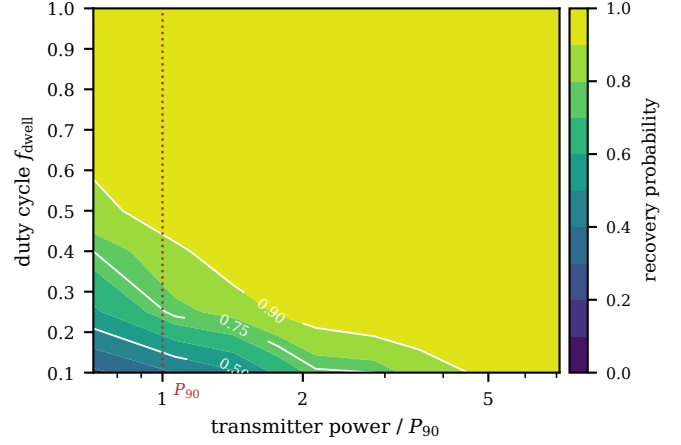
FIG. 9.— The duty-cycle selection function, measured. Recovery probability against transmitter power, in units of P_{90} , and duty cycle f_{\text{dwell}} , from 3 888 injection trials. The abscissa is in units of P_{90} , which is the pipeline’s nominal 5\sigma trigger multiplied by \times 2.29 for the spectral response and intra-integration smearing and then by \times 1.2 from the injection campaign, so a value of 1 here is \times 2.81 the trigger power and not the trigger power itself. The quoted P_{90} thresholds apply along the top of this plot. Recovery falls away below f_{\text{dwell}} \simeq 0.3 and a transmitter on a tenth of the time needs several times P_{90} to reach the same recovery, so the EIRP limits in this paper constrain persistent and high-duty-cycle emission and say progressively less about brief or scanning beacons. The dwell injections are zero-drift, so this selection function is measured for a stationary carrier and transferred to the drifting primary experiment; the joint drifting-and-intermittent cell is the one cell of Table 7 that remains unmeasured.
