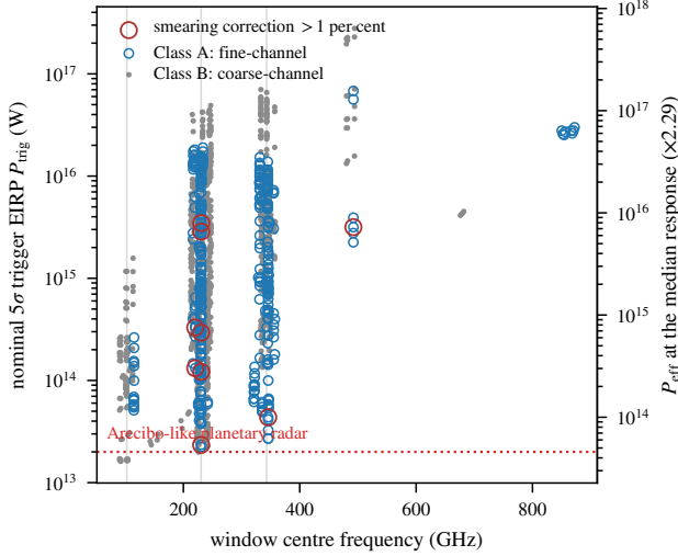
FIG. 10.— Two-dimensional sensitivity against window centre frequency for all 1655 searched windows, symbol by channelisation class, the axis along which completeness differs (Table 7). Left axis : the nominal trigger threshold P_{\text{trig}} , an internal detection statistic. Right axis : the effective threshold at the median response, P_{\text{eff}} = 2.29 P_{\text{trig}} , which is the power to compare with a transmitter (§4); the released per-window ratio P_{\text{eff, total}}/P_{\text{trig}} runs 1.33–3.98, so read a single window’s threshold from the catalogue and not from this axis. Red rings mark the 9 windows whose intra-integration smearing correction exceeds 1 per cent. Grey lines mark the Bands 3, 6 and 7 concentrations; dotted, the Arecibo 2.38-GHz EIRP benchmark, a power scale only. Note the two decades of scatter at fixed frequency: there is no single survey sensitivity.
