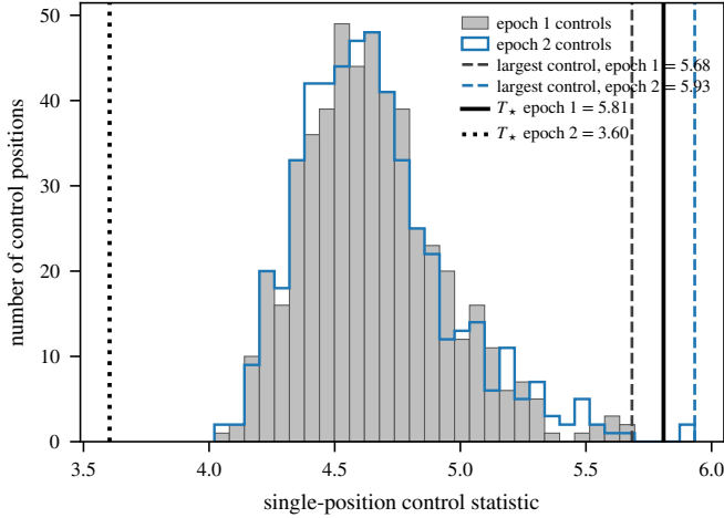
FIG. 14.— The CP–72 2713 Band 7 crossing inside its own control ensemble, in both executions. Histograms give the 512 single-position control statistics of that window in execution 1 (filled) and in the second block 2.05 h later (outline); the two agree, which is the evidence that the datasets are comparable. Vertical lines mark T_* and the largest control in each. In execution 2 the control annulus alone reaches 5.93, beyond the 5.81 that raised the flag, while the star falls to 3.60.
