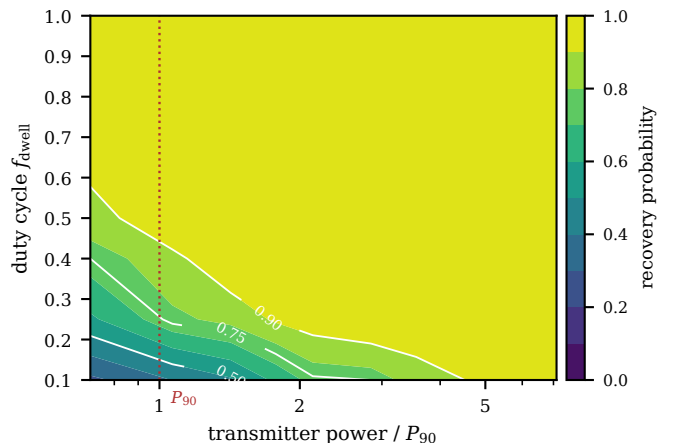
FIG. 8.— The duty-cycle selection function, measured. Recovery probability against transmitter power, in units of P_{90} , and duty cycle f_{\text{dwell}} , from 3888 injection trials. The abscissa is in units of P_{90} , which is the pipeline’s nominal trigger power multiplied by \times 2.29 for the spectral response and intra-integration smearing and then by \times 1.2 from the injection campaign, so a value of 1 here is \times 2.81 the trigger power and not the trigger power itself. The quoted P_{90} thresholds apply along the top of this plot. Recovery falls away below f_{\text{dwell}} \simeq 0.3 and a transmitter on a tenth of the time needs several times P_{90} to reach the same recovery, so the EIRP limits in this paper constrain persistent and high-duty-cycle emission and say progressively less about brief or scanning beacons. The dwell injections are zero-drift, so this selection function is measured for a stationary carrier and transferred to the drifting primary experiment; the joint drifting-and-intermittent cell is the one cell of Table 5 that remains unmeasured.
