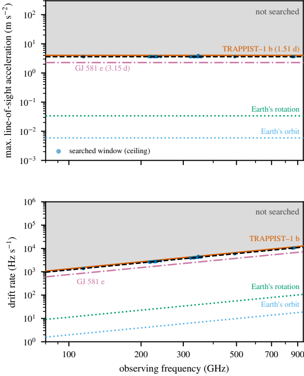
FIG. 11.— What the drift search does and does not reach, as a physical selection function. Upper : the drift ceiling of each of the 403 Class A windows (points), converted to the line-of-sight acceleration it corresponds to, |a| = c\dot{\nu}/\nu , against observing frequency; shaded above is unsearched. The boundary is flat because the grid was built at constant acceleration, 3.60 \text{ m s}^{-2} , and not at constant drift rate. Lower : the same boundary in the units the search works in, where it is not flat: the same 3.60 \text{ m s}^{-2} is 1.4 \text{ kHz s}^{-1} at 115 GHz and 10.5 \text{ kHz s}^{-1} at 872 GHz. Reference accelerations, all frequency-independent and so horizontal in the upper panel: Earth’s rotation ( 0.034 \text{ m s}^{-2} at the equator) and orbit ( 0.0059 \text{ m s}^{-2} ), which a terrestrial transmitter carries whether or not it intends to; the most demanding known planet of any target, TRAPPIST-1 b ( 4.00 \text{ m s}^{-2} ); and the next most demanding, GJ 581 e ( 2.27 \text{ m s}^{-2} ). TRAPPIST-1 b is the one case the grid does not contain, and it misses by 0.01 per cent (§6).
