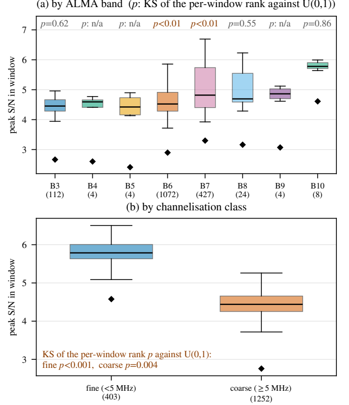
FIG. 12.— Exchangeability of the 512-position control ensemble by stratum, over 1655 windows. Boxes give the per-window control maximum, black diamonds the median on-star peak, and p the Kolmogorov–Smirnov test of the per-window rank against U(0,1) . (a) by ALMA band, with the window count under each label; (b) by channelisation class, fine (< 5 MHz) against coarse. The ensemble tracks the on-star statistic in every band, but both channelisation classes depart from uniformity: fine D = 0.150 , p < 10^{-4} over 403 windows, and coarse D = 0.050 , p = 0.004 over 1252. The departure is not the flagged windows’ doing — removing all 71 fine crossings leaves p = 0.002 — and §5.3.5 identifies the radial noise gradient as the cause.
