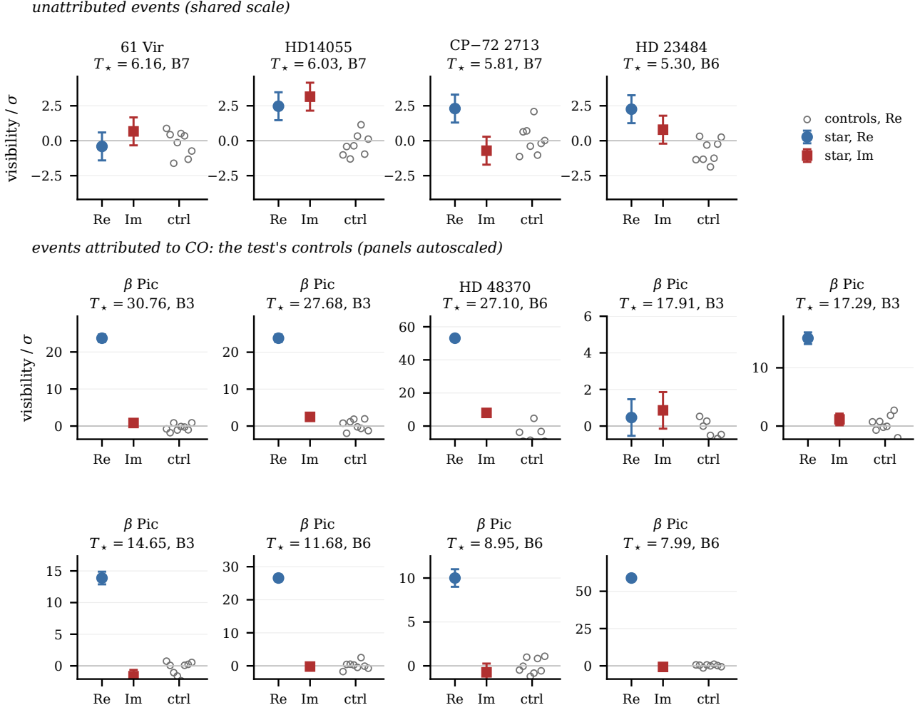
FIG. 7.— The visibility-domain test on all 13 stage-1 windows, one panel each. In units of the measurement uncertainty: the real part of the visibility phase-rotated to the stellar position (blue circle), which emission centred there makes positive and significant; its imaginary part (red square), which such emission leaves consistent with zero; and the real parts returned by eight control positions on the same annulus the image-plane screen uses (open circles). Top row: the 4 unattributed events, on one shared scale. None reaches 3\sigma ; 61 Vir does not beat its own controls; HD 14055 has a 3.2\sigma imaginary part, which a source centred on the star would not produce, but at this significance the test does not localise the excess either way. Lower rows: the 9 events attributed to carbon monoxide, which are the test's controls, each panel autoscaled because they reach 59\sigma . 7 are recovered at the stellar position; HD 48370 has a large real part but an imaginary part 7.9\sigma from zero, the displaced-source signature its foreground identification predicts; and one \beta Pictoris Band 3 block returns nothing, the one event whose test frequency had to be substituted from its siblings.
