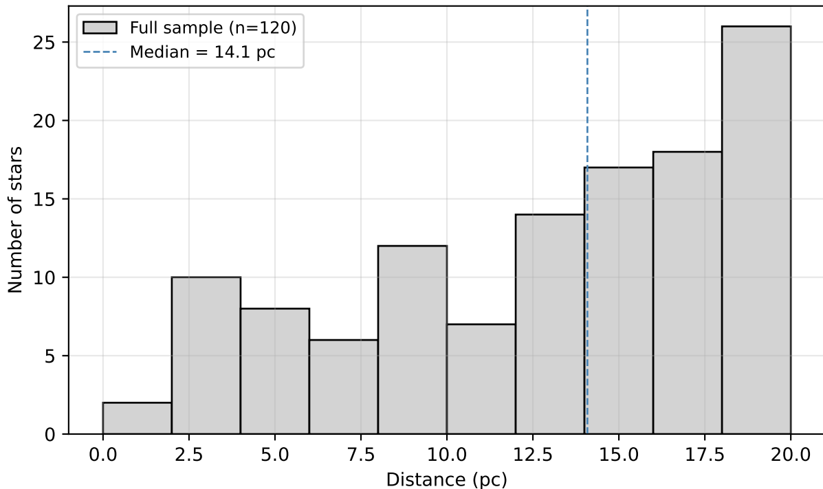
Volume-limited 20 pc sample: distance distribution
