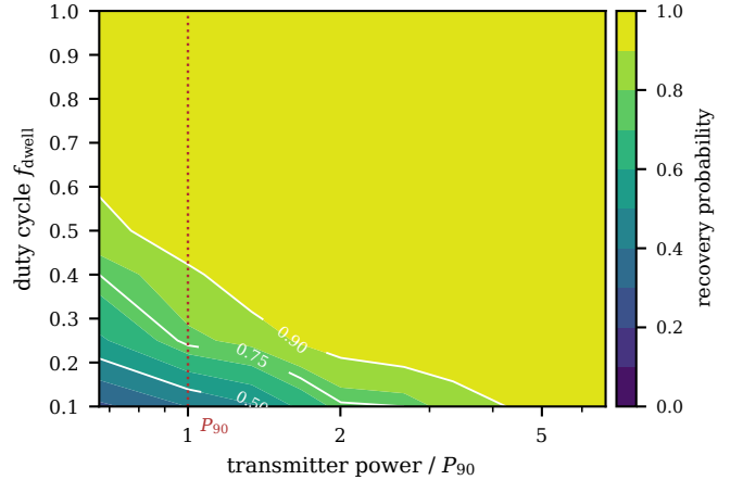
FIG. 6.— The duty-cycle selection function, measured. Recovery probability against transmitter power, in units of P_{90} , and duty cycle f_{\text{dwell}} , from 3888 injection trials. The abscissa is in units of P_{90} , the measured trigger completeness of §5.3, which for Class A is \times 3.0 the nominal trigger power. Recovery at f_{\text{dwell}} = 0.10 is 71 per cent for the fine class and 83 for the coarse, rising to 91 and 100 at f_{\text{dwell}} = 0.25 (Appendix G). The dwell injections are zero-drift, so this selection function is measured for a stationary carrier and transferred to the drifting primary experiment; the joint drifting-and-intermittent cell of Table 13 remains unmeasured.
