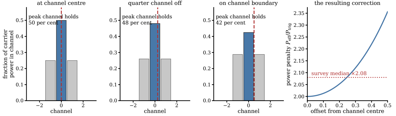
FIG. 9.— Why the nominal channel threshold is not the transmitter threshold. ALMA applies online Hanning smoothing by default, so an intrinsically unresolved carrier is spread over neighbouring channels and the peak channel holds only part of its power: half at a channel centre, 0.42 on a boundary (first three panels; blue is the peak channel, the dashed line the carrier). The search threshold is set in units of the channel noise, so the power a transmitter must radiate to reach it is larger than the nominal figure by the reciprocal of that fraction (right-hand panel). This is the whole of the difference between P_{\text{trig}} and P_{\text{eff}} .
