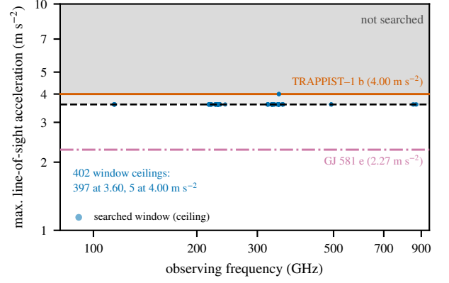
FIG. 4.— What the drift search reaches, as a physical selection function. Each point is the drift ceiling of one of the 402 Class A windows, converted to line-of-sight acceleration, |a| = c \dot{\nu}/\nu , against observing frequency; the shaded region above is unsearched. The boundary is flat because the grid was built at constant acceleration; in the units the search works in it is not, running 1.4 \text{ kHz s}^{-1} at 115 GHz to 10.5 \text{ kHz s}^{-1} at 872 GHz. The ceiling takes two values, 3.60 \text{ m s}^{-2} on 397 windows and 4.00 \text{ m s}^{-2} on the 5 TRAPPIST-1 ones, and it is each window's own ceiling that decides whether a given orbit is contained. The horizontal lines are the two most demanding known planets of any target, TRAPPIST-1 b ( 4.00 \text{ m s}^{-2} ) and GJ 581 e ( 2.27 \text{ m s}^{-2} ). Everything else of interest lies below the foot of the axis, including 30 of the 39 known planets in the sample and the two accelerations a transmitter on Earth would carry whether or not anyone intended it: the planet's rotation, 0.034 \text{ m s}^{-2} at the equator, a factor 106 below the ceiling, and its orbit, 0.0059 \text{ m s}^{-2} , a factor 607. TRAPPIST-1 b is the one planet above the default ceiling; it transits, so the edge-on case is the relevant one, and it lies above that ceiling for 29 per cent of its orbital phase and above the widened one for 1 per cent.
