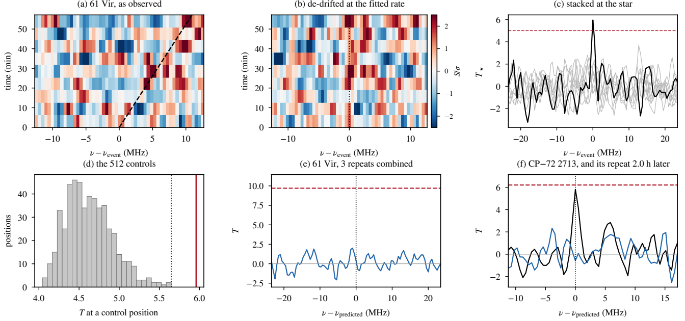
FIG. 8.— Why this survey reports no confirmed signal although it produced an interesting event. (a) The dynamic spectrum at 61 Vir’s position around the crossing at 346.313811 GHz, observed 2017 May 20, with the fitted drift of +3182 \text{ Hz s}^{-1} as the dashed track; the 225 integrations are binned into 9 and plotted in units of each bin’s noise. At 119 \pm 20 \text{ mJy} against 303 \text{ mJy} per integration the carrier is 0.39 standard deviations in any one of them and is invisible by eye, which is the point: the event exists only in the 38-minute coherent stack. (b) The same rows shifted by that drift, which carries the carrier 22 channels of 488.3 kHz across the observation; 8 of the 9 bins are positive at the marked channel. (c) The de-drifted stack at the star (black) and at the 8 control positions with retained dynamic spectra (grey), in units of its own noise; dashed, the trigger. (d) The same statistic at each of the 512 rank-screen control positions: the star reaches 5.96 (solid) against a highest control of 5.65 (dotted). (e) The 3 other blocks covering that cell in the star’s rest frame, combined, with zero at the predicted channel, which the frame transport moves between epochs; the nearest is 1.97 hours earlier than the discovery (2017 May 19), the farthest 3 days. A persisting carrier would have returned T = 9.7 (dashed) against 2.71 present, excluding it at 9.3\sigma . (f) The second event, CP-72 2713 at 344.269746 GHz: its discovery stack (black) and the same cell 2.05 hours later in a block 1.1 times deeper (blue), where a persisting carrier would have given T = 6.2 (dashed) against 3.60 measured. The inferred isotropic equivalent powers are 5.1 \times 10^{14} \text{ W} at 8.5 pc and 8.9 \times 10^{14} \text{ W} at 36.7 pc.
