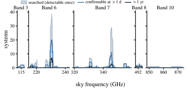
FIG. 10.— What could be searched against what could be confirmed. For the Class A experiment, against sky frequency: the number of systems toward which a carrier could have been detected once (grey), the number for which a second independent execution block more than a day later also covers that frequency (blue), and the same beyond a year (dark). One panel per populated ALMA band, widths in proportion to the frequency each contributes, as in Fig. 11. The grey curve has support 47.7 GHz of union bandwidth, the blue 23.3 GHz and the dark 8.5 GHz.
