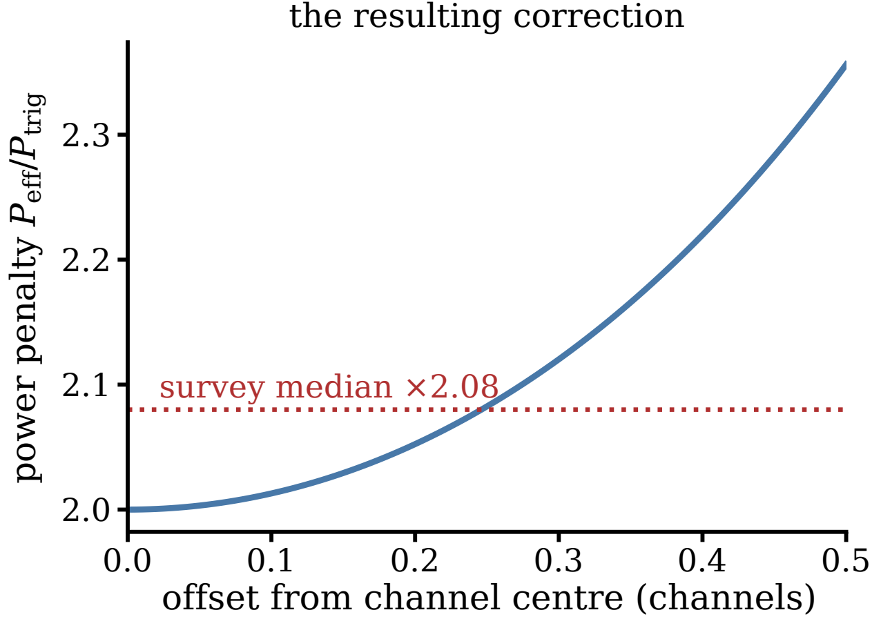
FIG. 12.— Why the nominal channel threshold is not the transmitter threshold. ALMA applies online Hanning smoothing by default, so an intrinsically unresolved carrier is spread over neighbouring channels and the peak channel holds only part of its power: half at a channel centre, 0.42 on a boundary (first three panels; blue is the peak channel, the dashed line the carrier). The search threshold is set in units of the channel noise, so the power a transmitter must radiate to reach it is larger than the nominal figure by the reciprocal of that fraction (right-hand panel). This is the whole of the difference between P_{\text{trig}} and P_{\text{eff}} .
