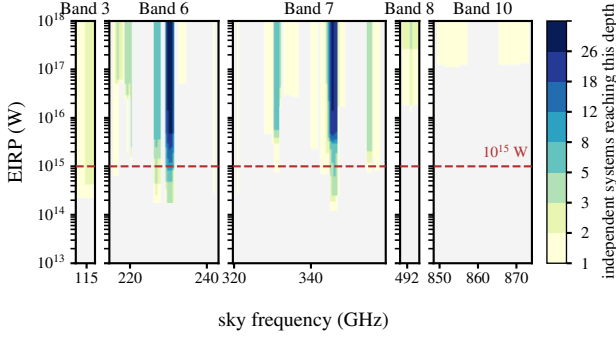
FIG. 11.— Where the experiment could have found something. Shading gives the number of independent systems that would have yielded a recovery at 90 per cent completeness for an unresolved carrier of the plotted EIRP at the plotted sky frequency; unshaded means none. One panel per populated ALMA band, with panel widths in proportion to the frequency each contributes: the 47.7 GHz Class A union is 26 disjoint islands spread across 114.0–873.1 GHz, so a single continuous abscissa would draw every island as a hairline. The dashed line is 1 \times 10^{15} W, at which 18.8 GHz of the union survives. Figure 3 shows where ALMA looked; this shows where the experiment was sensitive.
