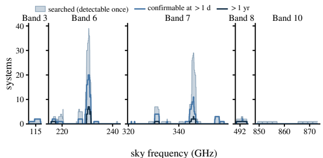
FIG. 10.— What could be searched against what could be confirmed. For the Class A experiment, against sky frequency: the number of systems toward which a carrier could have been detected once (grey), the number for which a second independent execution block more than a day later also covers that frequency (blue), and the same beyond a year (dark). One panel per populated ALMA band, widths in proportion to the frequency each contributes, as in Fig. 11. The grey curve has support 47.7 GHz of union bandwidth, the blue 23.3 GHz and the dark 8.5 GHz.
