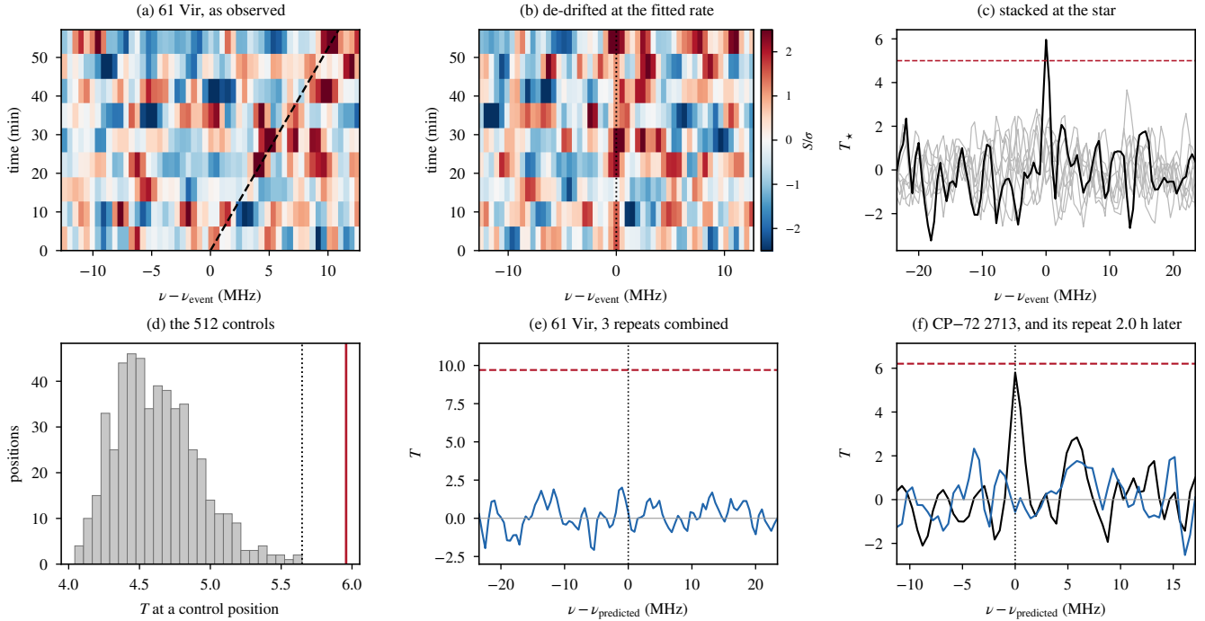
FIG. 8.— Why this survey reports no confirmed signal although it produced an interesting event. (a) The dynamic spectrum at 61 Vir’s position around the crossing at 346.313811 GHz, observed 2017 May 20, with the fitted drift of +3182 \text{ Hz s}^{-1} as the dashed track; the 225 integrations are binned into 9 and plotted in units of each bin’s noise. At 119 \pm 20 \text{ mJy} against 303 \text{ mJy} per integration the carrier is 0.39 standard deviations in any one of them and is invisible by eye, which is the point: the event exists only in the 38-minute coherent stack. (b) The same rows shifted by that drift, which carries the carrier 22 channels of 488.3 kHz across the observation; 8 of the 9 bins are positive at the marked channel. (c) The de-drifted stack at the star (black) and at the 8 control positions with retained dynamic spectra (grey), in units of its own noise; dashed, the trigger. (d) The same statistic at each of the 512 rank-screen control positions: the star reaches 5.96 (solid) against a highest control of 5.65 (dotted). (e) The 3 other blocks covering the same cell in the star’s rest frame, combined, with zero at the predicted channel, which the frame transport moves between epochs. The nearest is 1.97 hours earlier than the discovery (2017 May 19) and the farthest 3 days; a carrier persisting at the discovery flux would have returned T = 9.7 (dashed) and the largest value present is 2.71, so persistence is excluded at 9.3\sigma . (f) The second event, CP–72 2713 at 344.269746 GHz: its discovery stack (black) and the same cell 2.05 hours later in a block 1.1 times deeper (blue), where a persisting carrier would have given T = 6.2 (dashed) against 3.60 measured. The inferred isotropic equivalent powers are 5.1 \times 10^{14} \text{ W} at 8.5 pc and 8.9 \times 10^{14} \text{ W} at 36.7 pc.
