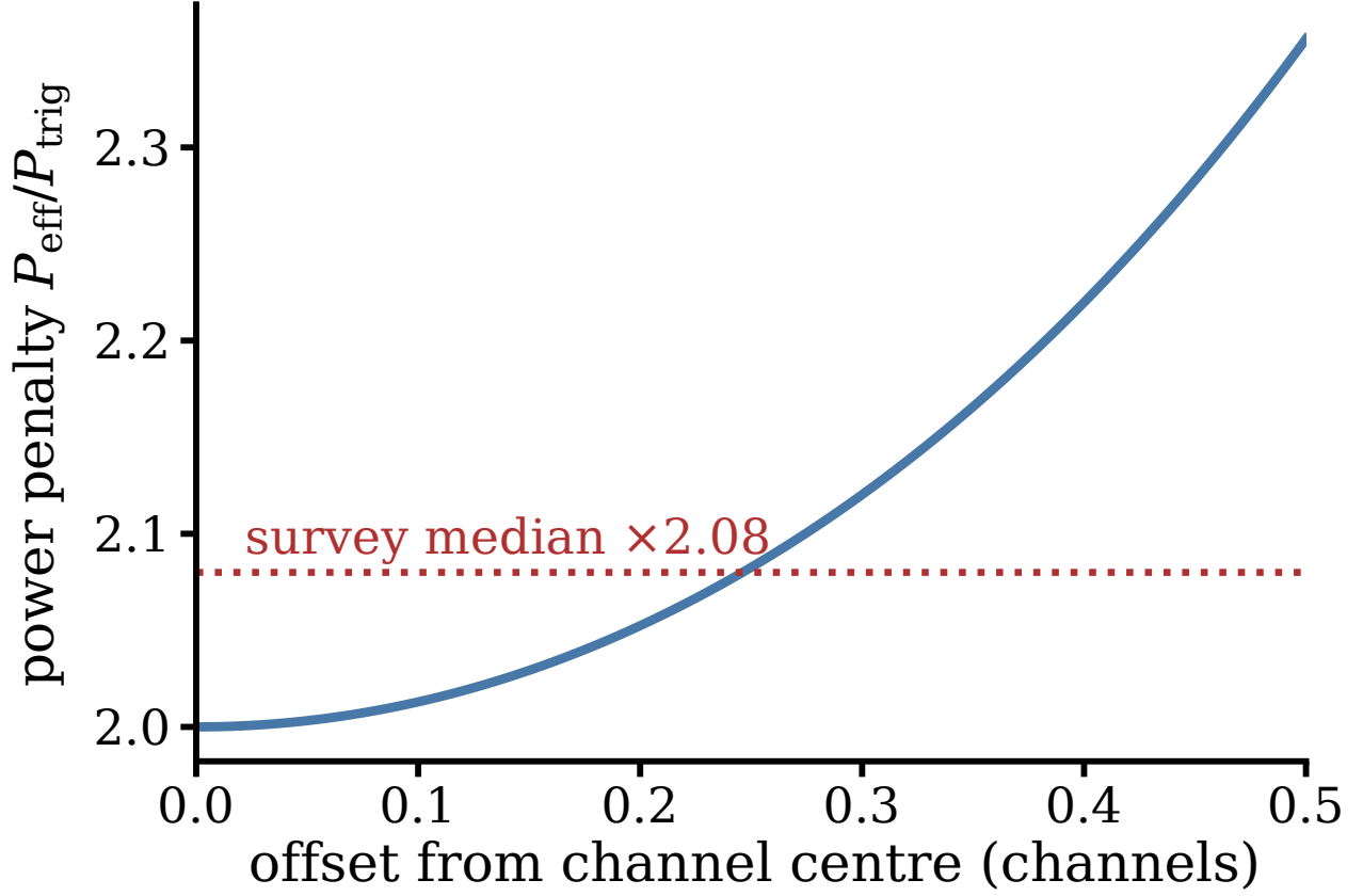
FIG. 12.— Why the nominal channel threshold is not the transmitter threshold. ALMA applies online Hanning smoothing by default, so an intrinsically unresolved carrier is spread over neighbouring channels and the peak channel holds only part of its power: half at a channel centre, 0.42 on a boundary (first three panels; blue is the peak channel, the dashed line the carrier). The search threshold is set in units of the channel noise, so the power a transmitter must radiate to reach it is larger than the nominal figure by the reciprocal of that fraction (right-hand panel). This is the whole of the difference between P_{\text{trig}} and P_{\text{eff}} .
