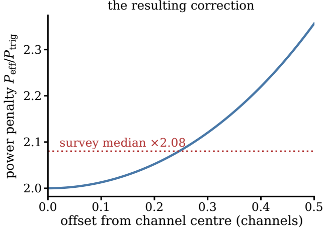
FIG. 10.— Why the nominal channel threshold is not the transmitter threshold. ALMA applies online Hanning smoothing by default, so an intrinsically unresolved carrier is spread over neighbouring channels and the peak channel holds only part of its power: half at a channel centre, 0.42 on a boundary. The threshold is set in units of the channel noise, so the power a transmitter must radiate to reach it is larger than the nominal figure by the reciprocal of that fraction, plotted here against where in the channel the carrier falls. This is the whole of the difference between P_{\text{trig}} and P_{\text{eff}} .
