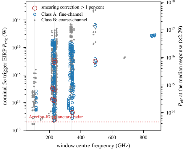
FIG. 10.— Two-dimensional sensitivity against window centre frequency for all 1655 searched windows, symbol by channelisation class, the axis along which completeness differs (Table 13). Left axis : the nominal trigger threshold P_{\text{trig}} , an internal detection statistic. Right axis : the effective threshold at the median response, P_{\text{eff}} = 2.29 P_{\text{trig}} , which is the power to compare with a transmitter (§4); the per-window ratio P_{\text{eff, total}}/P_{\text{trig}} runs 1.33–3.98, so a single window’s threshold should be read from the catalogue, not from this axis. Red rings mark the 9 windows whose smearing correction exceeds 1 per cent; dotted, the Arecibo 2.38-GHz benchmark. Note the two decades of scatter at fixed frequency: there is no single survey sensitivity.
