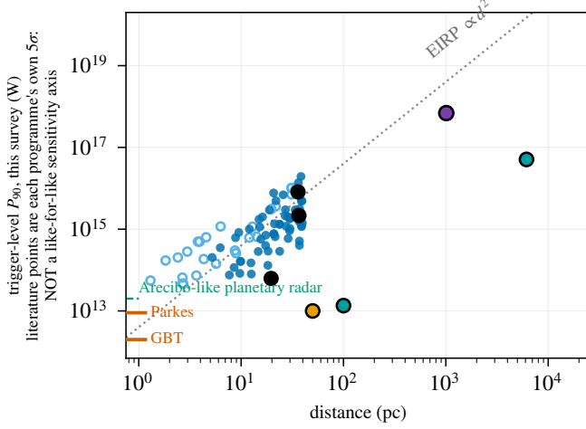
FIG. 11.— EIRP against distance for this survey and for published centimetre-wave searches. Blue: this survey, plotted as the trigger-level P_{90} for the deepest window per star; orange: Enriquez et al. (2017); aqua: Margot et al. (2023); violet: Mason et al. (2024); left-edge ticks: Price et al. (2020). Grey dotted: \text{EIRP} \propto d^2 at constant received flux. Green dashed: the Arecibo 2.38-GHz benchmark, a power scale only. The vertical coordinates are not comparable completeness limits: each programme's value is its own threshold statistic over its own channel width, and those widths differ by about seven orders of magnitude (Fig. 1).
