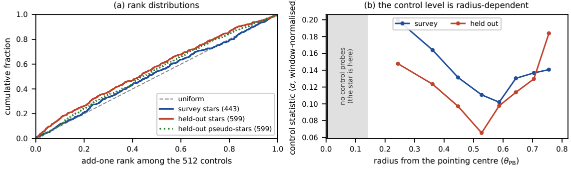
FIG. 4.— Why the spatial control ensemble is a calibrated screen and not an exchangeable rank test. (a) add-one rank of the star among its 512 controls, for the survey and for the held-out windows carrying no attributed line: both lie above the uniform diagonal. The dotted curve is the pseudo-stars , control positions at the inner edge of the annulus ranked against the other controls, which contain no star and are displaced just as far (§5.3), so the displacement is instrumental. (b) the control statistic itself against radius from the pointing centre, in units of each window’s own noise scale. It is lowest at mid-annulus and rises towards both edges; the shaded strip inside 0.14 \theta_{PB} holds no control probe at all, and that is where the star sits (median 0.0035 \theta_{PB} ).
