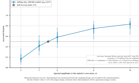
FIG. 8.— Measured injection recovery on real ALMA data, fine-channel configuration. Recovery C(A, f_{\text{drift}}) rises with amplitude for drifting carriers; static and near-static ones fail the frozen criterion, and boundary-straddling tones can fail its peak-drift clause while still being detected. Coarse configurations are not plotted: under the same criterion they recover nothing, withdrawn in the text as an artefact of the criterion.
