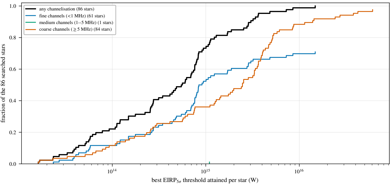
(b) per-star achieved sensitivity
