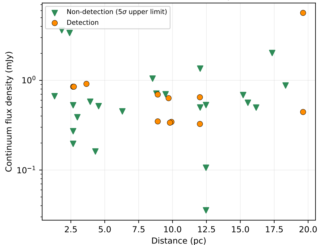
Continuum sensitivity
