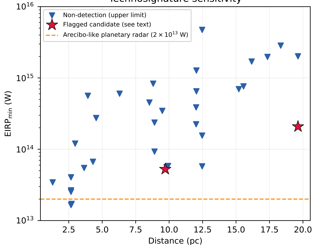
Technosignature sensitivity
