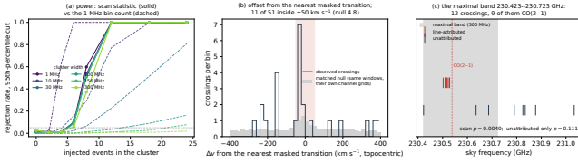
FIG. 16. — (a) Measured rejection rate of the 1 MHz multiplicity statistic (dashed) and of the scan statistic (solid) against the number of injected events, by cluster width, at a threshold fixed beforehand from the channel-grid null. The old statistic is blind to anything wider than a channel. (b) Each crossing's velocity offset from the nearest masked transition, with a null drawn from the same windows' own channel grids: 11 of 51 inside \pm 50 \text{ km s}^{-1} against 4.7 expected. (c) The maximal band, 230.423–230.723 GHz, with its 12 members coloured by attribution and CO(2→1) marked.
