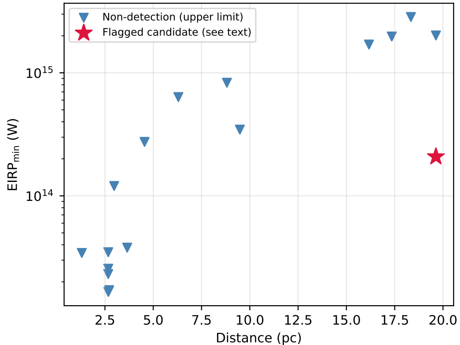
Technosignature sensitivity
