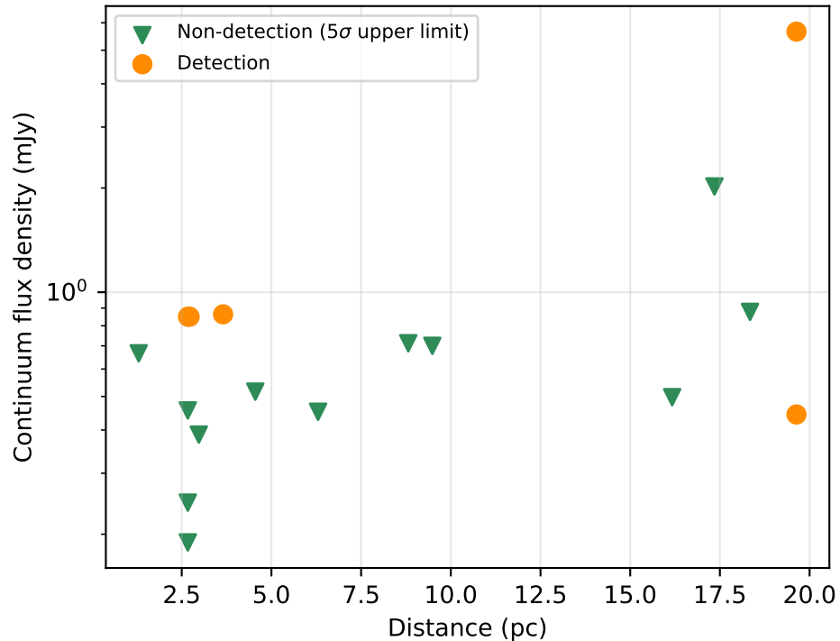
Continuum sensitivity
