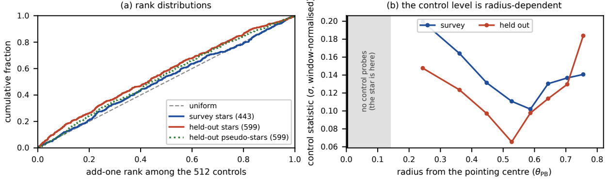
FIG. 4.— Why the spatial null is a calibrated screen and not an exchangeable rank test. (a) add-one rank of the star among its 512 controls, for the survey and for the held-out windows carrying no attributed line: both lie above the uniform diagonal. The dotted curve is the pseudo-stars , control positions at the inner edge of the annulus ranked against the other controls, which contain no star and are displaced just as far (§5.3), so the displacement is instrumental. (b) the control statistic itself against radius from the pointing centre, in units of each window’s own noise scale. It is lowest at mid-annulus and rises towards both edges; the shaded strip inside 0.14\theta_{PB} holds no control probe at all, and that is where the star sits (median 0.0035\theta_{PB} ).
